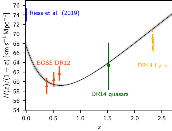
Fig. 16. Comoving Hubble parameter as a function of redshift. The grey bands show the 68% and 95% confidence ranges allowed by Planck TT,TE,EE+lowE+lensing in the base- \Lambda CDM model, clearly showing the onset of acceleration around z = 0.6 . Red triangles show the BAO measurements from BOSS DR12 (Alam et al. 2017), the green circle is from BOSS DR14 quasars (Zarrouk et al. 2018), the orange dashed point is the constraint from the BOSS DR14 Ly \alpha auto-correlation at z = 2.34 (de Sainte Agathe et al. 2019), and the solid gold point is the joint constraint from the Ly \alpha auto-correlation and cross-correlation with quasars from Blomqvist et al. (2019). All BOSS measurements are used in combination with the Planck base-model measurements of the sound horizon r_{\text{drag}} , and the DR12 points are correlated. The blue point at redshift zero shows the inferred forward-distance-ladder Hubble measurement from Riess et al. (2019).
