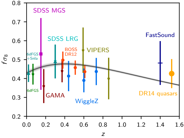
Fig. 14. Constraints on the growth rate of fluctuations from various redshift surveys in the base- \Lambda CDM model: dark cyan, 6dFGS and velocities from SNe Ia (Huterer et al. 2017); green, 6dFGS (Beutler et al. 2012); purple square, SDSS MGS (Howlett et al. 2015); cyan cross, SDSS LRG (Oka et al. 2014); dark red, GAMA (Blake et al. 2013); red, BOSS DR12 (Alam et al. 2017); blue, WiggleZ (Blake et al. 2012); olive, VIPERS (Pezzotta et al. 2017); dark blue, FastSound (Okumura et al. 2016); and orange, BOSS DR14 quasars (Zarrouk et al. 2018). Where measurements are reported in correlation with other variables, we here show the marginalized posterior means and errors. Grey bands show the 68% and 95% confidence ranges allowed by Planck TT, TE, EE + lowE + lensing.
