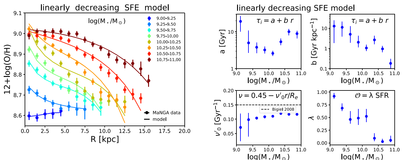
Figure 9. Left: Same as Fig. 7, but using the linearly decreasing SFE model. Right: Same as Fig. 8, but using the linearly decreasing SFE model. The parameter \nu_0 denotes the linear slope of the SFE and is compared to the median value obtained analysing the data from Bigiel et al. (2008) for a small sample of local star-forming galaxies.
