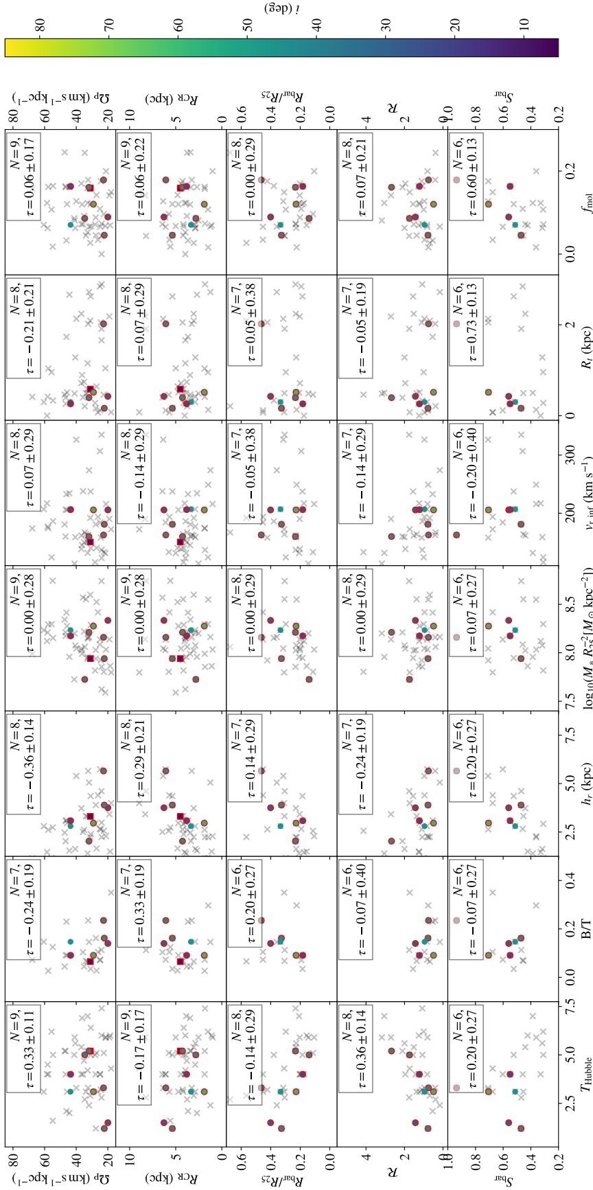
Figure 12. From top to bottom: the pattern speed, co-rotation radius, bar radius, \mathcal{R} , and bar strength versus, from left to right: the Hubble morphological type, bulge-to-total flux ratio, galaxy disk scale length, stellar mass divided by R_{25}^2 , asymptotic rotation velocity, galaxy rotation turnover radius, and molecular gas fraction. Points are coloured by the inclination of the galaxy, galaxies with bars shown as circles, and galaxies without as squares, and galaxies with noted spiral arms are highlighted in red. In each subplot, the number of points, N , and the Kendall \tau correlation is given, along with its associated uncertainty. We also plot well-constrained PHANGS-ALMA values as grey crosses.
