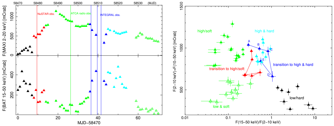
Figure 1. Left panel: the MAXI (upper) and Swift/BAT (lower) light curves of MAXI J1631–479, both with 1 day binning. Vertical lines indicate the time of the NuSTAR , ATCA and INTEGRAL observations. See text for details. Right panel: the hardness-intensity diagram with each point corresponding to 1 day: on the horizontal axis we show the ratio F_{(15-50\text{ keV})}^{BAT}/F_{(2-10\text{ keV})}^{MAXI} and in the vertical axis the total flux F_{(15-50\text{ keV})}^{BAT} + F_{(2-10\text{ keV})}^{MAXI} . Colored points indicate the different time intervals. Capitals letters indicate the time evolution of the hardness-intensity data during this transition, with A being the starting of the transition and E the end.
