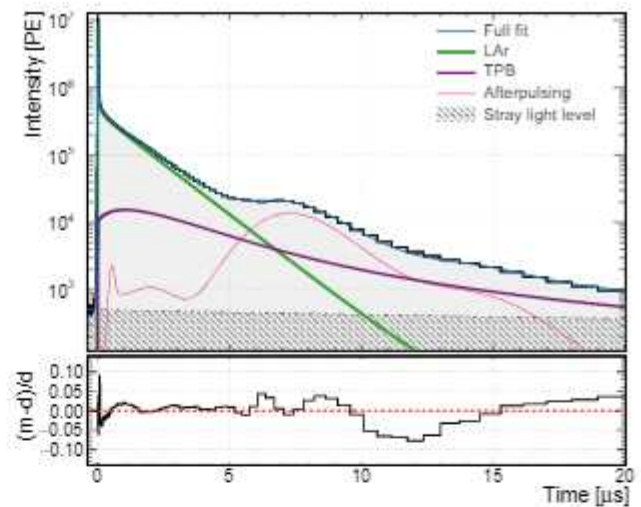
Fig. 6 From 0.2 \mu\text{s} to 5 \mu\text{s} , the pulseshape is dominated by the LAr scintillation light. The region from 5 \mu\text{s} to 10 \mu\text{s} is dominated by PMT afterpulsing. Starting at approximately 13 \mu\text{s} , the TPB delayed emission becomes significant. While the total event length in standard DEAP data is 16 \mu\text{s} , the analysis window on which PSD as well as event energy and position reconstruction is based is -0.03 \mu\text{s} to 10 \mu\text{s} with respect to the event peak
