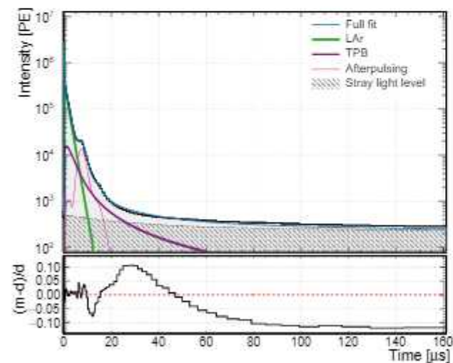
Fig. 5 At time scales beyond 15 \mu\text{s} , the pulseshape is dominated by the delayed TPB emission. At approximately 30 \mu\text{s} , the intensity of TPB emission has declined to the point where it is equal to the intensity of left-over late light from previous events
