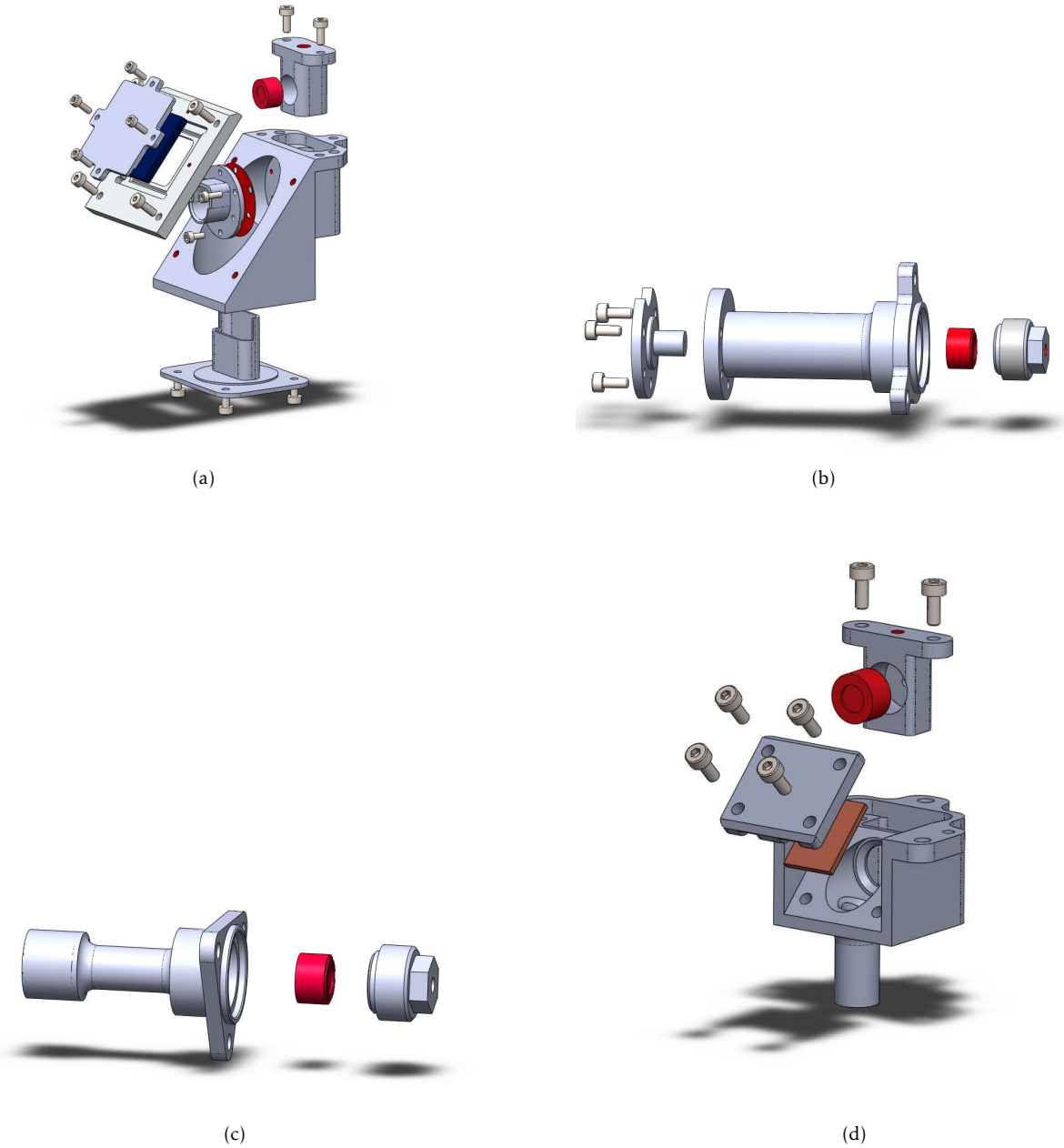
Figure 6. CAD models of the calibration set. All sources are derived from capsules containing an ^{55}\text{Fe} nuclide: (a) Cal A is the polarized source. It is un-collimated and provides simultaneous polarized X-rays at 3.0 keV and 5.9 keV, (b) Cal B is an unpolarized collimated 5.9 keV source, (c) Cal C is a broad 5.9 keV source for flat field illumination, (d) Cal D is a broad 1.7 keV source for gain and spurious modulation check-out
