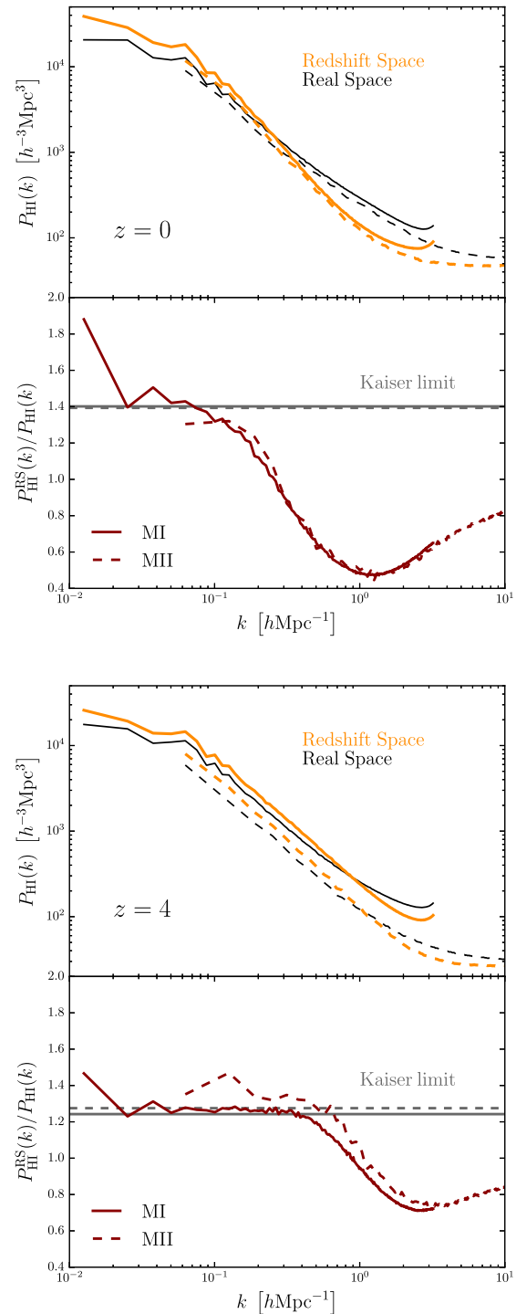
Figure 19. Comparison between the H I power spectrum computed in real space (black) and in redshift space (orange), for the MI (solid) and MII (dashed) simulations (dashed lines), for z = 0 (top) and z = 4 (bottom panels). In the lower sub-panel of each panel, we show the Kaiser limit for both the MI (grey solid) and the MII (grey dashed), computed as in equation (9), and compared to what is measured in simulations.
