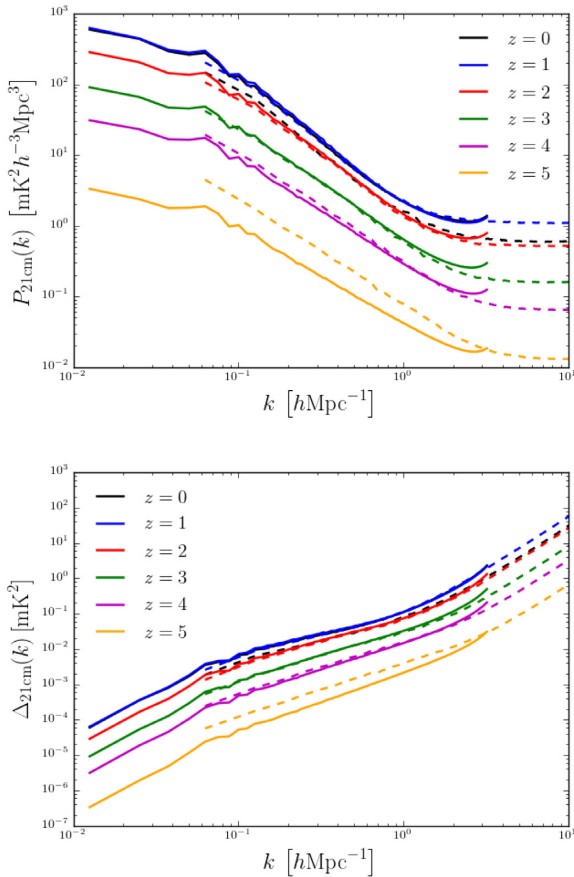
Figure 20. The power spectrum of the 21 cm signal P_{21\text{ cm}}(k) (top panel) and the \Delta_{21\text{ cm}}(k) \equiv P_{21\text{ cm}}(k)k^3/2\pi^2 (bottom panel) as predicted from the MI (solid lines) and the MII (dashed lines), at different redshifts (from z = 0 to 5, colour coded as in legend).
