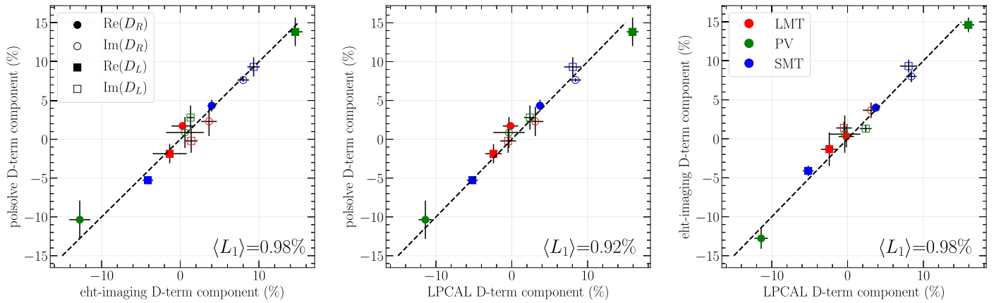
Figure 20. Example one-to-one software comparisons of the campaign-average D-term estimates for LMT, PV, and SMT. Left panel: comparison of eht-imaging estimates against polsolve estimates. Middle panel: comparison of LPCAL estimates against polsolve estimates. Right panel: comparison of LPCAL estimates against eht-imaging estimates. The L_1 norm is averaged over the left/right and real/imaginary components of the D-terms and over all three EHT stations shown. See Section 4.2 for a discussion of the D-term L_1 norm values between eht-imaging/polsolve/LPCAL and THEMIS/DMC.
