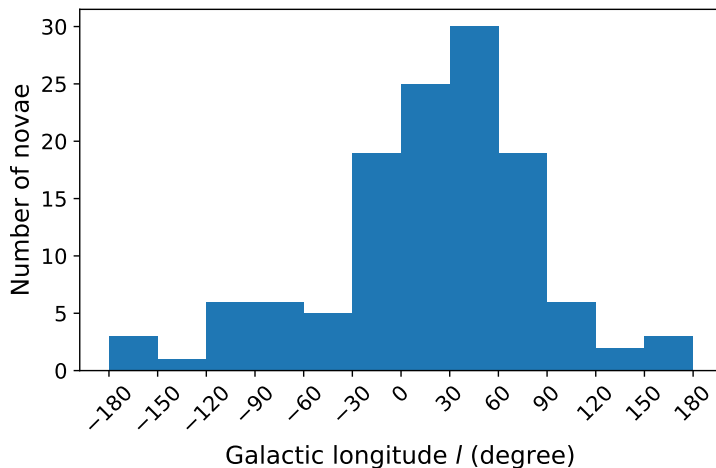
Fig. 6 Distribution of the galactic longitudes of novae inside the Milky Way. Data from Özdönmez et al (2018)
