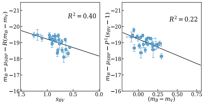
Fig. 3. Luminosity correlation plots for the SBF sample: the absolute magnitude ( m_B - \mu_{\text{SBF}} ) corrected for the color vs. the LC stretch parameter ( left panel ), and the absolute magnitude corrected for the LC stretch vs. color ( right panel ). The correlation parameters are evaluated using the Bayesian analysis described in Sect. 3.4. The solid black lines show the best-fit model obtained with the MCMC sampling. The R^2 score (coefficient of determination) of the fit is shown in the top right.
