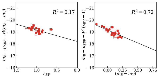
Fig. 5. Luminosity correlation parameters for the SHOES sample: the absolute magnitude ( m_B - \mu_{\text{SBF}} ) corrected for the color vs. the LC stretch parameter ( left panel ), the absolute magnitude corrected for the LC stretch vs. color ( right panel ). The correlation parameters are evaluated using the Bayesian analysis. The solid black lines show the best-fit model obtained with the MCMC sampling. The R^2 score (coefficient of determination) of the fit is shown in the top right.
