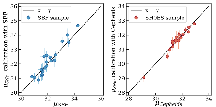
Fig. 12. Distance modulus comparisons of the two local calibration samples. The left plot shows the comparison between directly measured SBF distances ( \mu_{SBF} , given in Table 1) for the SBF sample, with the SNe distances estimated using the SBF calibration of the cosmological redshift-cut sample of 96 SNe as described in Section 3. The right plot shows similar comparison for the SHOES sample, comparing the measured Cepheid distances (from R16) with the distances estimated using the Cepheid calibration of the cosmological redshift-cut sample. In both cases we find a good one-to-one agreement.
