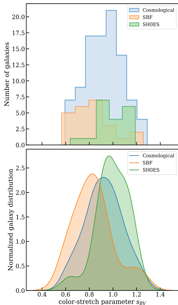
Fig. 2. Number of galaxies (top panel) and the normalized density distribution (bottom panel) of the s_{BV} parameter values of SNe Ia of the three data samples used in this work: the SBF calibration sample, the SH0ES calibration samples, and the cosmological sample.
