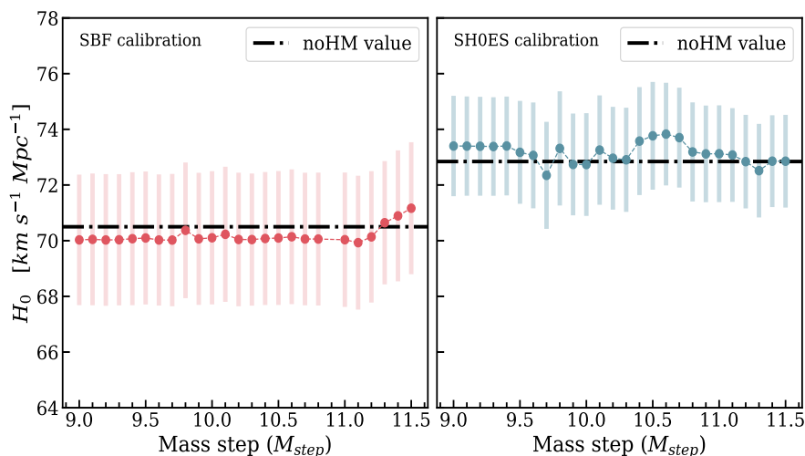
Fig. 9. H_0 values estimated including the step mass correction in the calibration at different values of M_{step} . The SBF calibration with a step mass correction decreases the H_0 value by \sim 0.5\% almost consistently at each M_{step} except at the extreme end. However, for the SH0ES calibration, step based correction gives fluctuating values. The lowest value is found at M_{step} = 9.7 and is 0.7\% lower than the noHM value and the highest is found for M_{step} = 10.6 , which is 1.4\% higher than the noHM value of H_0 .
