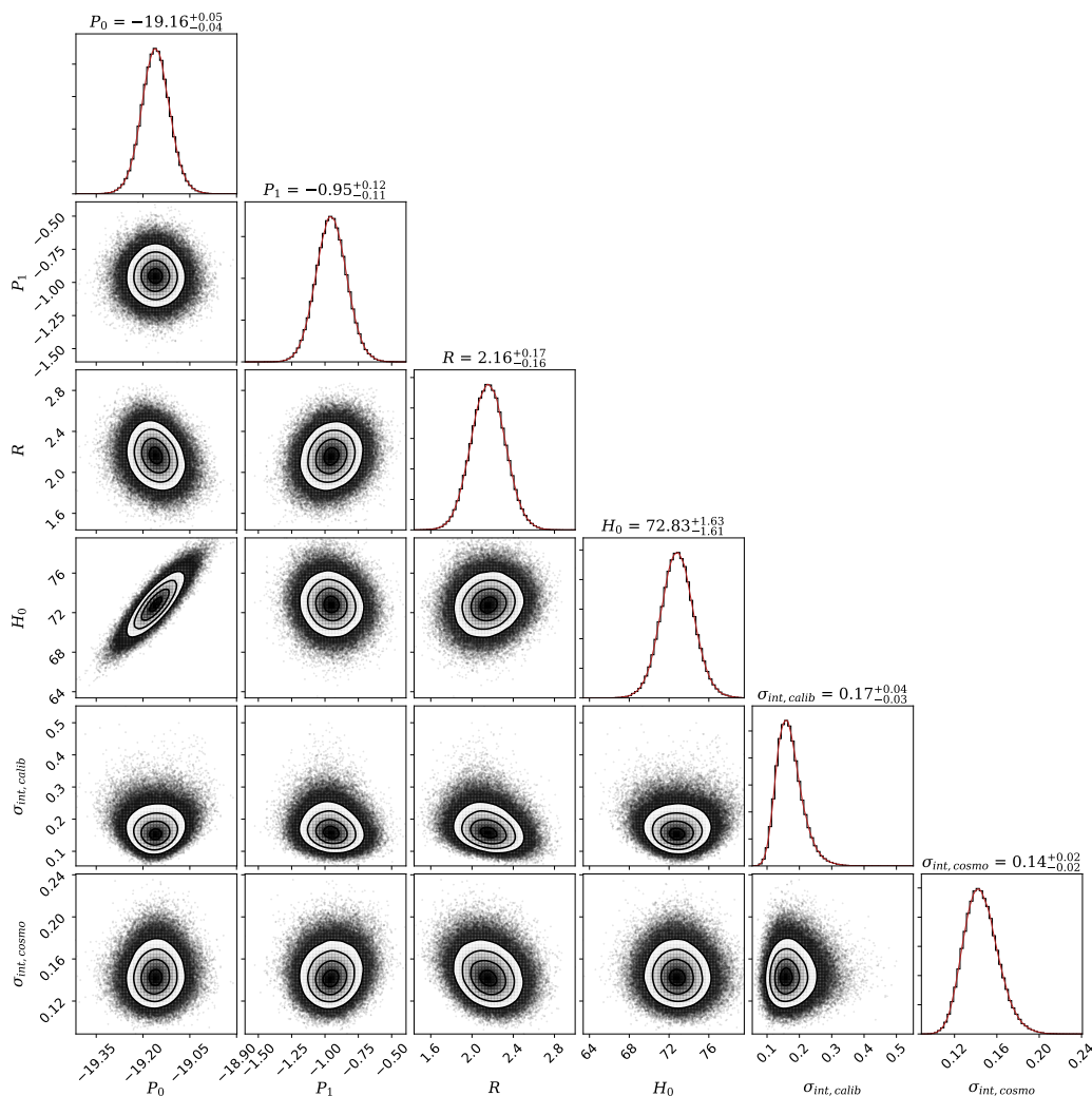
Fig. 6. Corner plot showing posterior distributions for the parameters P_0 , P_1 , R and H_0 along with the intrinsic scatter obtained using the SH0ES sample with the redshift-cut cosmological sample. The title on each histogram shows the median value of the respective posterior distribution. The luminosity correction does not include any dependence on host galaxy stellar mass.
