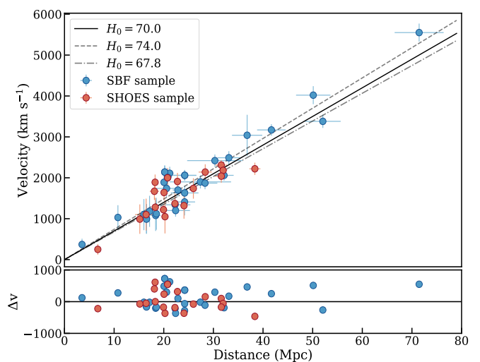
Fig. 13. Nearby Hubble diagram for galaxies with SBF and Cepheid distance measurements. The recessional velocities for all galaxies are corrected for peculiar motions with the CF model following Carrick et al. (2015). As a reference, also shown is the Hubble law for the values of the Hubble constant of H_0 = 70.0 \text{ km s}^{-1} \text{ Mpc}^{-1} (solid line), H_0 = 74.0 \text{ km s}^{-1} \text{ Mpc}^{-1} (dashed line) and H_0 = 67.8 \text{ km s}^{-1} \text{ Mpc}^{-1} (dot-dashed line). The bottom panel shows the residuals for both the SBF and SHOES samples calculated assuming a H_0 of 70 \text{ km s}^{-1} \text{ Mpc}^{-1} .
