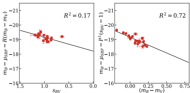
Fig. 5. Luminosity correlation parameters for the SHOES sample: the absolute magnitude ( m_B - \mu_{SBF} ) corrected for the color vs. the LC stretch parameter (left panel), the absolute magnitude corrected for the LC stretch vs. color (right panel). The correlation parameters are evaluated using the Bayesian analysis. The solid black lines show the best-fit model obtained with the MCMC sampling. The R^2 score (coefficient of determination) of the fit is shown in the top right.
