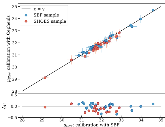
Fig. 11. Distance moduli of the SNe Ia belonging to the two local samples (SBF and SHOES) estimated using the Cepheid (y-axis) or the SBF (x-axis) as calibrators. The two calibrations used here do not include the cosmological sample in the analysis. It does not include the host galaxy mass correction. For a visual comparison, the line x=y is plotted. The bottom panel shows the residual difference among the distances calibrated by Cepheid and SBF, \Delta\mu = \mu^{Ceph} - \mu^{SBF} .
