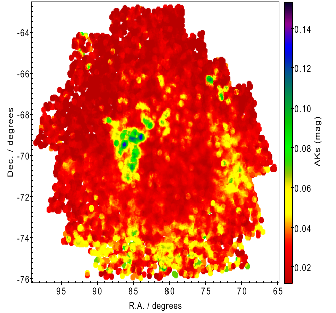
Figure 4. K_s -band absorption map derived from the RRL stars. The position of each RRL was re-binned to a circle of 30 arcsec in diameter.
