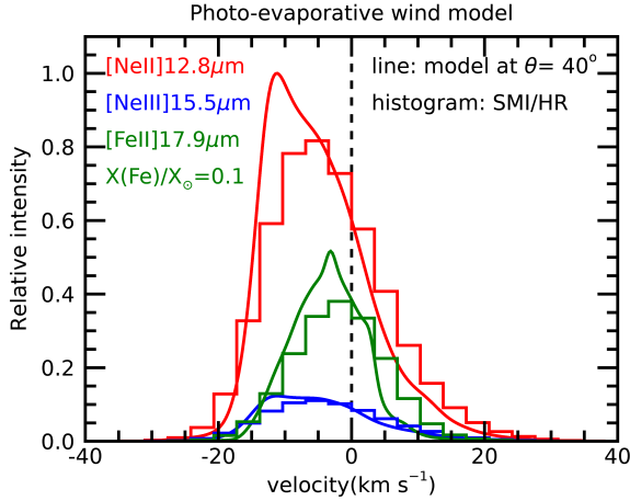
Figure 7. Expected profiles of the [Ne II]12.8 \mu\text{m} (red), [Ne III] 15.5 \mu\text{m} (blue) and [Fe II]17.9 \mu\text{m} (green) lines excited in a X-ray induced photoevaporative wind, based on the models of Picogna et al. (2019) and the calculations of Weber et al. (2020). Histograms show how the lines are seen by the SMI instrument. An iron abundance ten times smaller than solar has been assumed, taking into account the expected Fe depletion onto dust grains.
