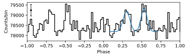
Figure 2. One of the 45 min segments of Obs. 12 folded with the period P_{\text{init}} = 0.08936694 s. The blue line shows two Gaussian functions used to fit the main optical peaks. The average 1\sigma error bar is shown on the top left.
