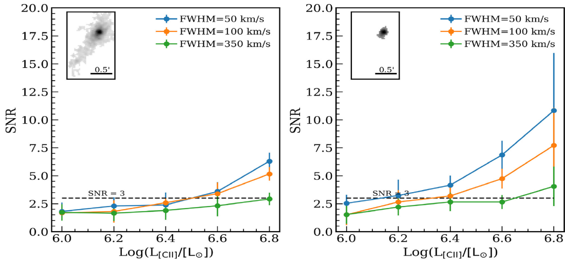
Figure A1. Mock ALMA observations of D1 for various assumptions on the line width, on the luminosity and spatial distribution of the [C II] emission. In the left- and right-hand panels D1 is modelled as an extended and point-like source, respectively, with the adopted light distribution reported in the top left-hand inset of each figure. The plots show the S/N as a function of [C II] luminosity, computed assuming a linewidth of 50 \text{ km s}^{-1} (blue solid lines and solid circles), 100 \text{ km s}^{-1} (orange lines), and 350 \text{ km s}^{-1} (green lines). For further details, see Appendix A.
