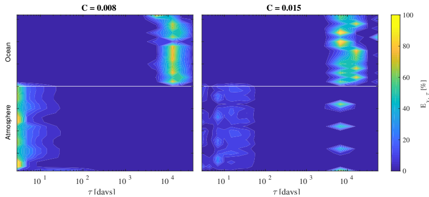
Figure 3. Relative contribution (in percentage) E_{\chi,\tau} of each variable \chi = \{\psi_{a,i}, \theta_{a,i}, \Psi_{o,i}, T_{o,i}\} in dependence on the mean timescale \tau . Left and right panels refer to the two values of the friction coefficient C = 0.008 and C = 0.015 , respectively. The white line separates the atmospheric variables from the oceanic ones.
