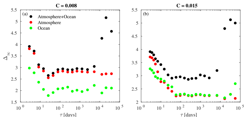
Figure 10. Multifractal width \Delta_\infty at different timescales \tau_j for reconstructions of MIMFs summing up from j = 1 to N_j ( D_q^{\sum_j} ) for (a) C = 0.008 and (b) C = 0.015 . The different colors refer to the full system (atmosphere+ocean, black circles), only the atmosphere (red circles), and only the ocean (green circles), respectively.
