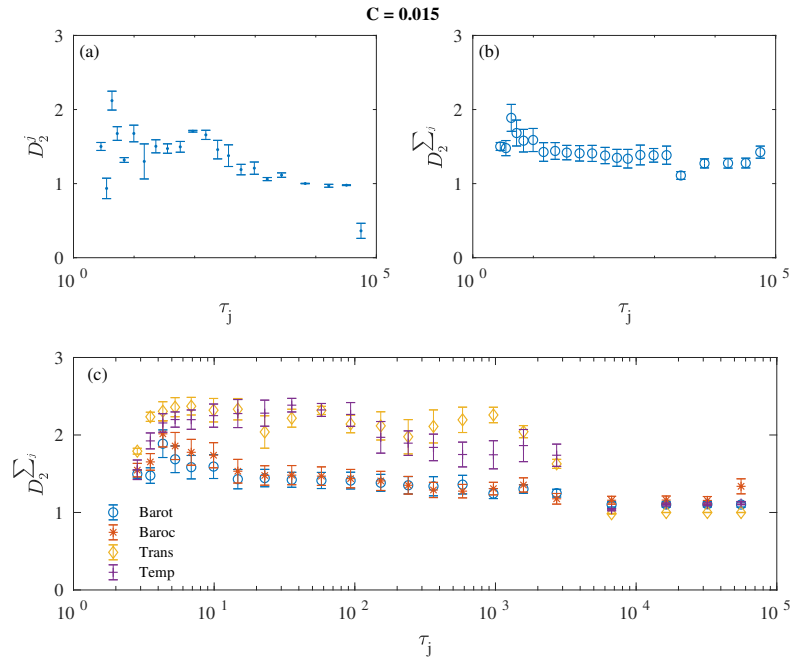
Figure 6. Same as in Fig. 5, but for C = 0.015 .
