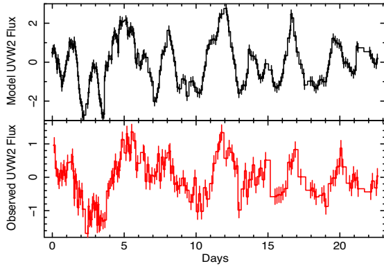
Figure 13. The model (upper panel) and observed (lower panel) UUVW2 light curves from Fig. 12 following subtraction of the mean level derived from smoothing with a 5 d wide boxcar.
