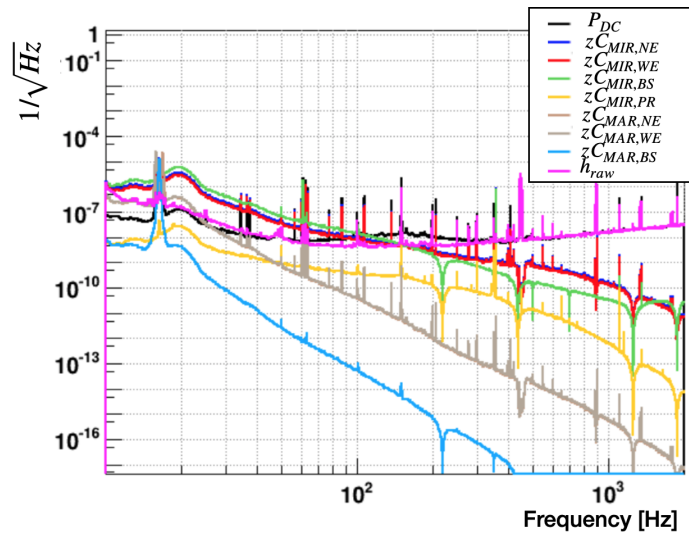
Figure 12. Contributions of the mirrors longitudinal controls to the reconstructed signal h_{raw} in O. Black curve is the amplitude spectral density of the dark fringe signal P_{DC} . Pink curve is the amplitude spectral density of h_{raw} purple in watt units. The other curves are the contribution of the various controls zC_i in the same units.
