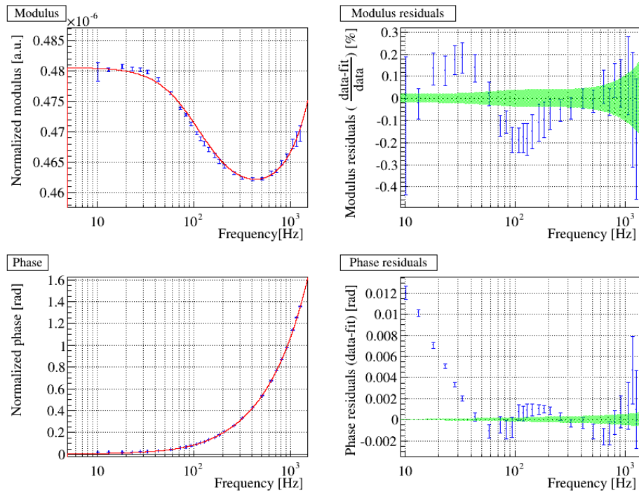
Figure 4. NE mirror actuator response normalized by the simple pendulum mechanical model. On the left, the measurements are represented in blue and the fit is drawn in red. Modulus is given in m/V and phase in rad. The modulus and the phase are fitted simultaneously. On the right, the residuals are shown. The green area represents the uncertainties given back by the fitted model, taking into account parameter covariance.
