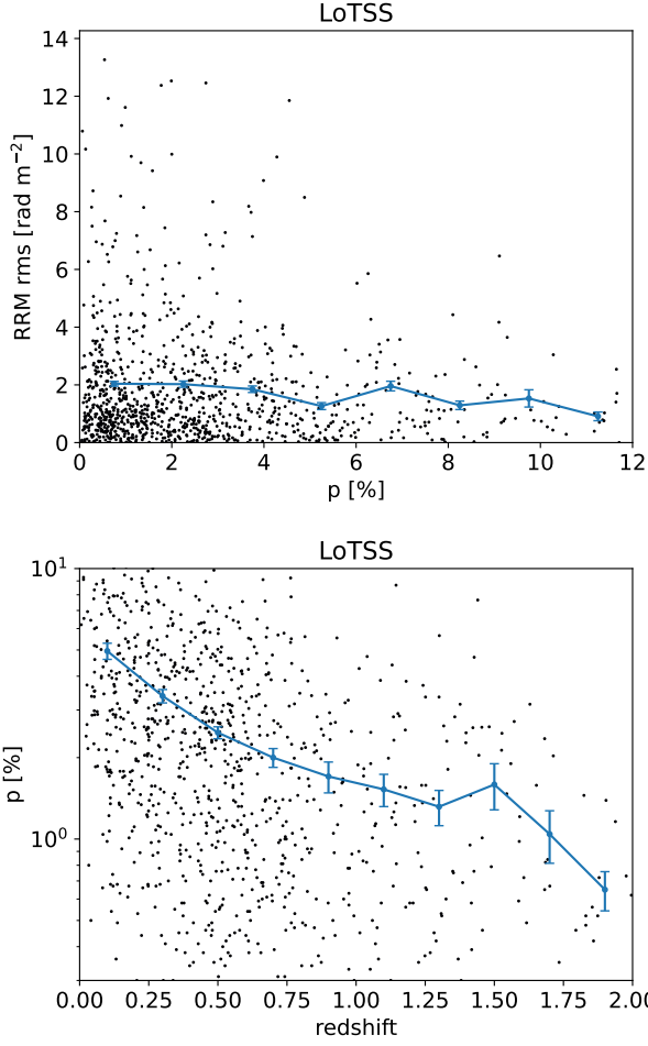
Figure 6. Top: RRM rms deviation as a function of fractional polarization p of the LoTSS sample (solid line). Individual |\text{RRM}| s are also reported (dots). Bottom: Mean of the fractional polarization p as a function of z of the LoTSS sample (solid line). Individual fractional polarizations are also reported (dots).
