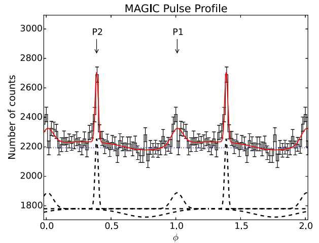
Figure 1. MAGIC 50–400 GeV pulse profile of the Crab pulsar (Aleksic et al. 2012b), along with the fitting function I (red solid line; see text for details). The black dashed lines represent the Gaussian components of I , while the blue dotted line is the background level. P1 and P2 are the main pulse and interpulse, respectively. The adopted number of bins per period is 51.
