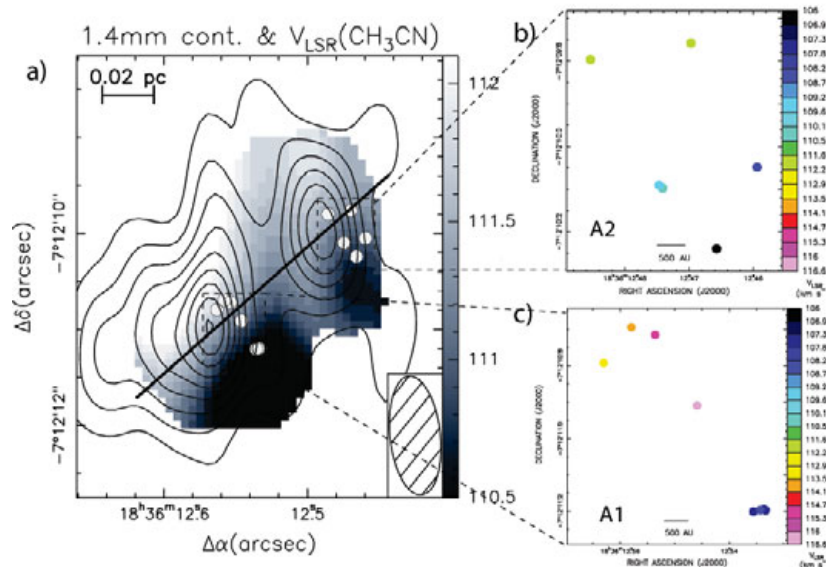
Figure 1. a) Map of the CH 3 CN (12 → 11) line peak velocity towards G24 A, with the contour levels in kilometers per seconds indicated in the wedge to the right of the panel (Beltrán et al. 2004); overlaid on the CH 3 CN velocity map, is shown the contour map of the 1.4 mm continuum emission ( solid lines ) and the positions of the CH 3 OH 6.7 GHz masers ( filled spheres ); the straight black line represents the axis of the molecular outflow observed with PdBI in 12 CO(1–0) by Furuya et al. (2002). b) and c) Positions and line-of-sight velocities of the 6.7 GHz maser features observed towards the subcore A2 and A1, respectively, with the colors (see online version) denoting different line-of-sight velocities, according to the scale on the right-hand side of the panels.
