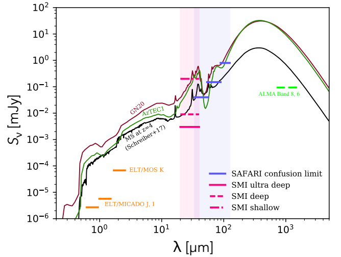
Figure 14. Fits to the observed SEDs of: the z\approx 4 starburst galaxy GN20 (purple); and the z=4.34 sub-mm galaxy AzTEC-1 (green). These are both fitted with the models of Efstathiou & Siebenmorgen (2009), and the average z\approx 4 MS galaxy observed by Schreiber et al. (2017) with ALMA (black). Pink horizontal lines represent the limits of the Ultra-Deep, Deep and Shallow reference surveys planned with SMI and described in Section 4. The blue horizontal lines show the confusion flux for a 2.5-m telescope in the SAFARI bands. For comparison, ALMA ( 3\sigma , 5 hr in Band 8 and 20 min in Band 6: green horizontal lines), ELT/MOS and ELT/MICADO (3 hr, orange horizontal lines) detection limits are shown.
