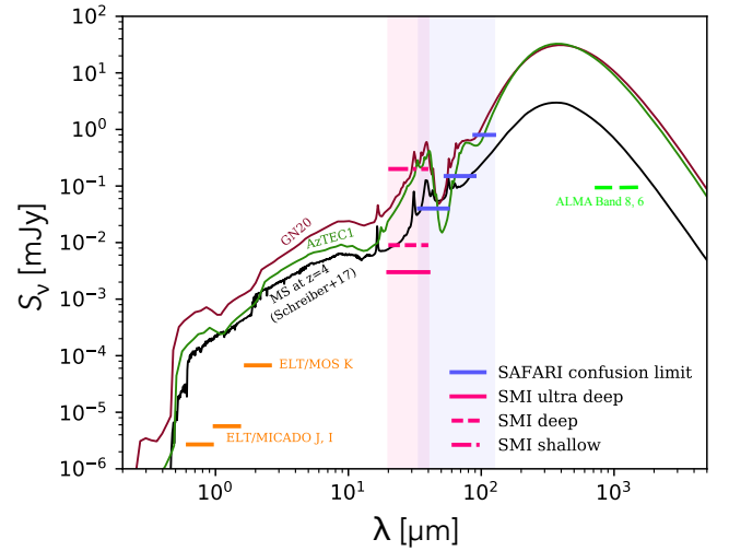
Figure 14. Fits to the observed SEDs of: the z \simeq 4 starburst galaxy GN20 (purple); and the z=4.34 sub-mm galaxy AzTEC-1 (green). These are both fitted with the models of Efstathiou & Siebenmorgen (2009), and the average z \simeq 4 MS galaxy observed by Schreiber et al. (2017) with ALMA (black). Pink horizontal lines represent the limits of the Ultra-Deep, Deep and Shallow reference surveys planned with SMI and described in Section 4. The blue horizontal lines show the confusion flux for a 2.5-m telescope in the SAFARI bands. For comparison, ALMA ( 3\sigma , 5 hr in Band 8 and 20 min in Band 6: green horizontal lines), ELT/MOS and ELT/MICADO (3 hr, orange horizontal lines) detection limits are shown.
