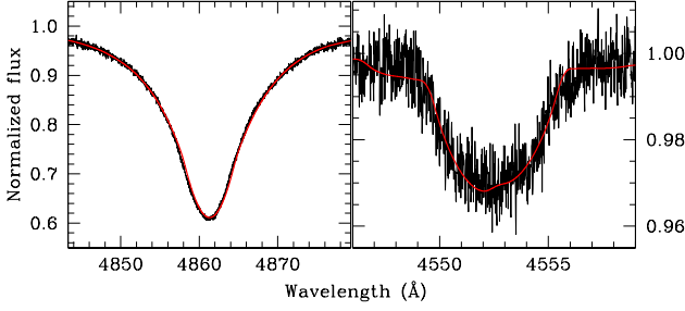
Figure 2. The left panel shows the comparison between observed (HARPS-N) and computed H \beta . The right panel shows the comparison between observed and synthetic Si III line at \lambda = 4552.622 Å.
