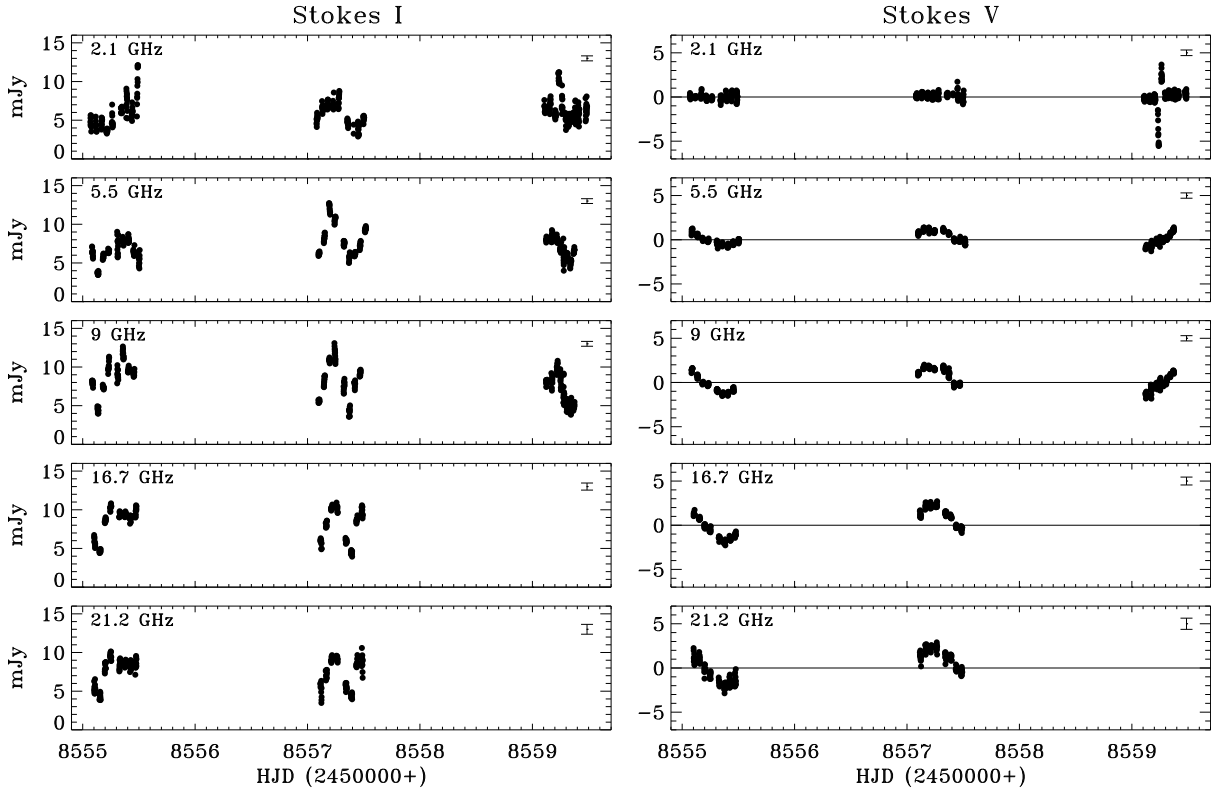
Figure 1. Multi-wavelength ATCA radio measurements of \rho Oph A. Left panels refer to the total intensity (Stokes I ) measurements. Right panels show the circularly polarized intensity (Stokes V ). The representative error bars of the radio measurements are displayed in the right upper corner of each panel.
