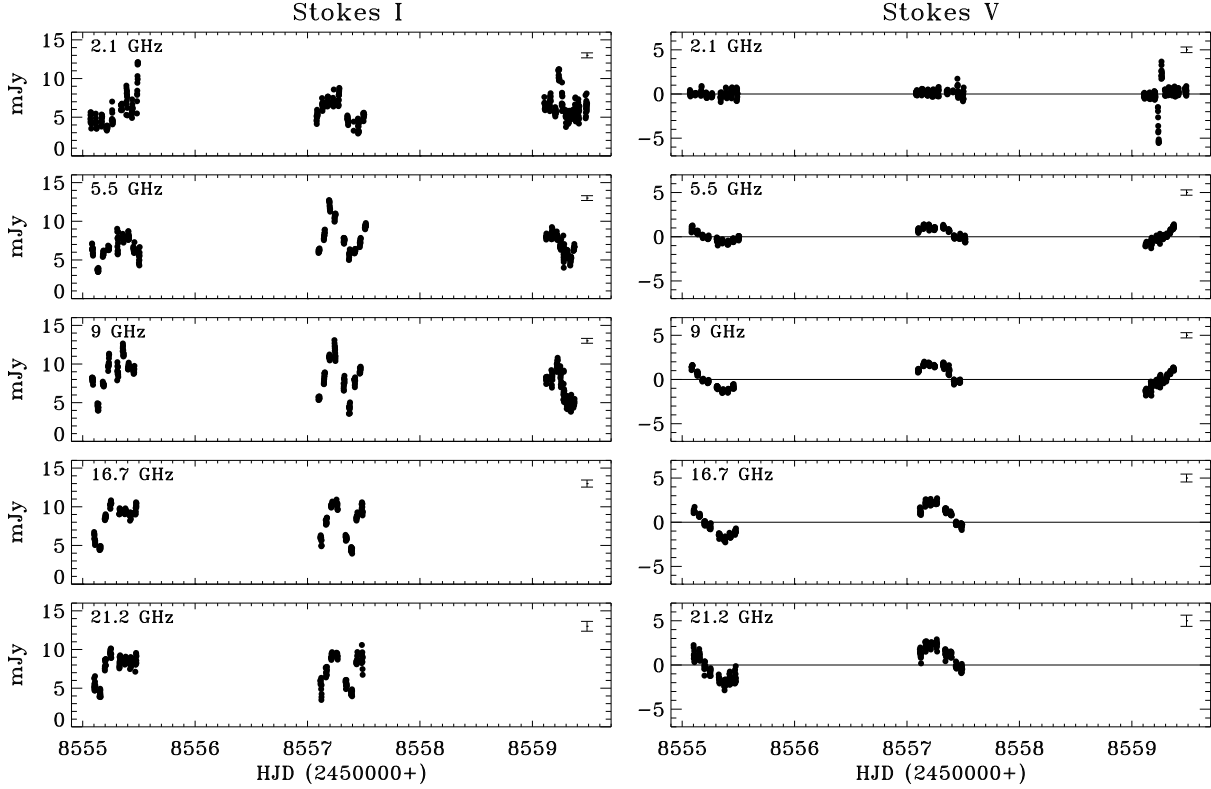
Figure 1. Multi-wavelength ATCA radio measurements of \rho Oph A. Left panels refer to the total intensity (Stokes I ) measurements. Right panels show the circularly polarized intensity (Stokes V ). The representative error bars of the radio measurements are displayed in the right upper corner of each panel.
