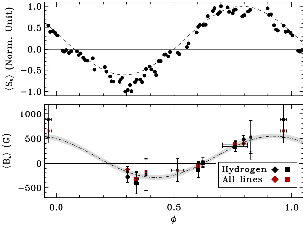
Figure 8. Top panel: average of the circularly polarized radio emission of \rho Oph A at \nu \geq 5.5 GHz. Each single band dataset was normalized to the their extrema (positive/negative). The normalized data, averaged within a phase bin 0.01 large, are displayed using the filled dots. The dashed line is the sinusoidal fit of the data. Bottom panel: effective magnetic field curve of \rho Oph A. The open symbols refer the \langle B_z \rangle measurements obtained from lower quality spectra (quality threshold S/N > 1000). The gray area represents the envelope of the sinusoidal curves compatible with the errors of the data fit parameters.
