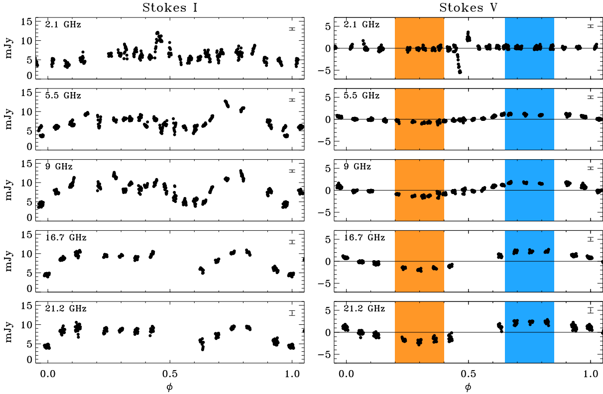
Figure 5. Rotational variability of the multiwavelength \rho Oph A radio emission. Left panels: total intensity (Stokes I ). Right panels: circularly polarized intensity (Stokes V ). The vertical orange bars (centred at \phi = 0.3 ) highlight the range of phases where Stokes V is clearly negative at \nu \geq 5.5 GHz; the light-blue bars (centred at \phi = 0.75 ) refer to the phase range with Stokes V > 0 .
