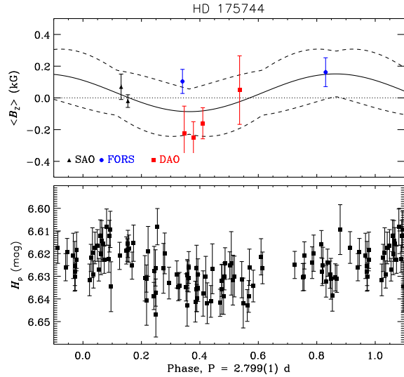
Figure C30. Top : \langle B_z \rangle measurements of HD 175744 folded with the rotation period inferred from Hipparcos photometry ( Bottom ). The harmonic fit to \langle B_z \rangle is performed to the combined magnetic dataset.
