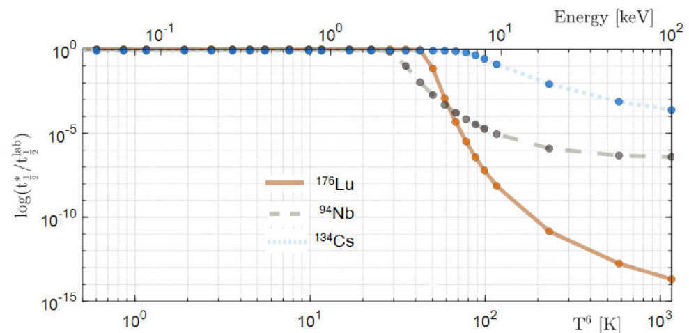
Figure 7. Theoretical estimates (based on [27]) of the ^{176}\text{Lu} , ^{134}\text{Cs} , and ^{94}\text{Nb} ratios of stellar half-life to terrestrial half-life dependence as a function of plasma temperature T^6 [ 10^6 K] (Energy [keV]) at densities of PANDORA’s plasmas ( 10^{12} \text{ cm}^{-3} ). The red line corresponds to the trend of ^{176}\text{Lu} . The dashed, gray line shows the trend of ^{94}\text{Nb} , while the blue, dotted line indicates the trend of ^{134}\text{Cs} .
