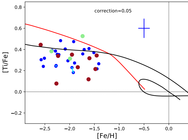
Fig. 11. [Ti/Fe] versus [Fe/H] abundances measured in the MINCE stars; the details are the same as Fig. 6.
