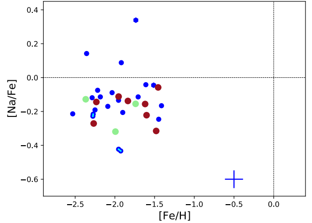
Fig. 13. [Na/Fe] versus [Fe/H] abundances measured in the MINCE stars; the details are the same as Fig. 6, but without the lines of models.
