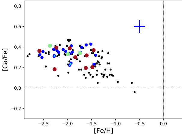
Fig. 10. [Ca/Fe] versus [Fe/H] abundances measured in the MINCE stars; the plot is the same as Fig. 9, but without the lines of models and with the results by Ishigaki et al. (2012) for halo stars (black dots).
