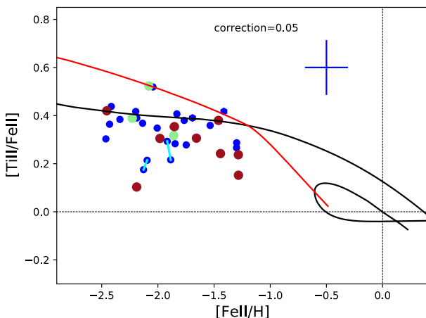
Fig. 12. [Ti\ II/Fe\ II] versus [Fe\ II/H] abundances measured in the MINCE stars; the details are the same as Fig. 6.
