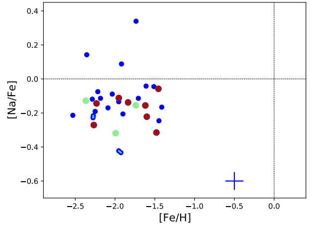
Fig. 13. [\text{Na}/\text{Fe}] versus [\text{Fe}/\text{H}] abundances measured in the MINCE stars; the details are the same as Fig. 6, but without the lines of models.
