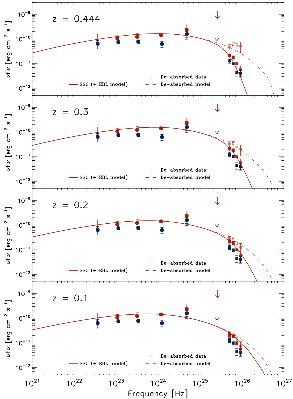
Figure 7. SSC models for redshifts z = 0.444, 0.3, 0.2, and 0.1 from top to bottom. The Fermi -LAT and VERITAS data points follow the same convention used in the paper to distinguish between flare (red) and dark run (blue) data points. In each panel, the EBL-absorbed model is shown as a solid red line and the de-absorbed model as a dashed red line. De-absorbed VERITAS flare points are shown as open squares. In all cases, the optical depth values from Franceschini et al. (2008) are used. The best agreement between the model and the data is achieved when the source is located at z = 0.2 – 0.3 . For lower redshifts, the model spectrum is systematically too hard, while at z = 0.444 , the model spectrum is too soft.
