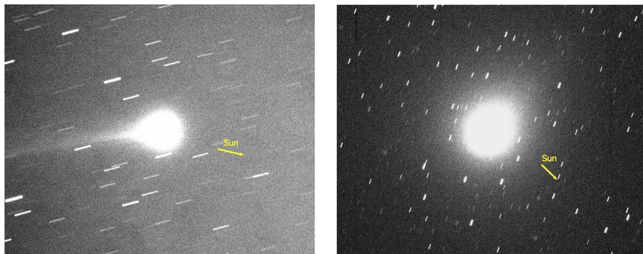
Figure 2. Images of 45P/HMP (left) on 2016 December 28 taken at the Farn telescope and 46P/Wirtanen (right) on 2018 December 9 taken at the Remote Observatory Atacama Desert (ROAD) telescope. Both represent the closest day to perihelion that we have for each comet. The arrows represent the projected solar direction on the plane of the sky, and represent 50,000 km and 10,000 km, respectively. In both images, north is up and east is to the left.
