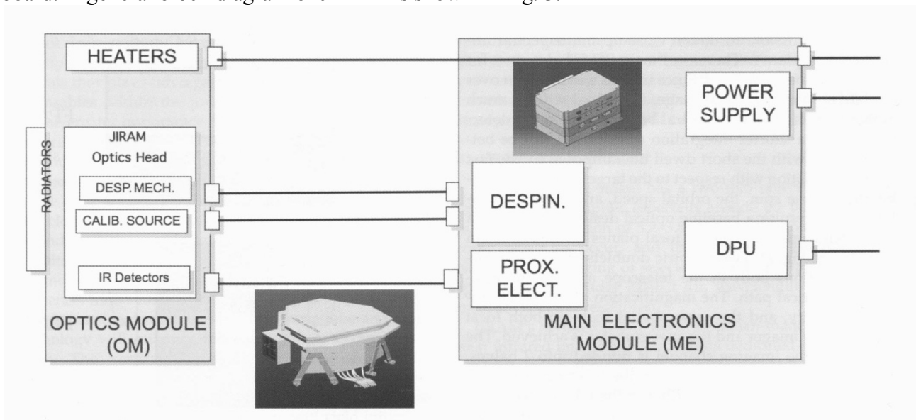
Figure 4: General block diagram of JIRAM.
