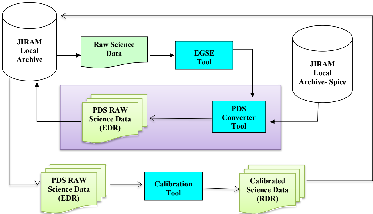
Figure 8: Jiram processing data.
