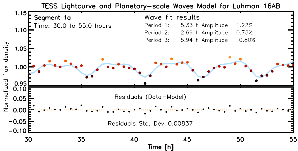
Figure 9. Upper panel: Segment 1a of the Luhman 16 lightcurve (minus the long-term trend) and the planetary-scale waves model (blue curve). Bottom panel: residuals (data–model) and the model. The planetary-scale waves model reproduces the evolution of the lightcurve well with fitted period values that are fully consistent with those found in the Lomb–Scargle analysis.
