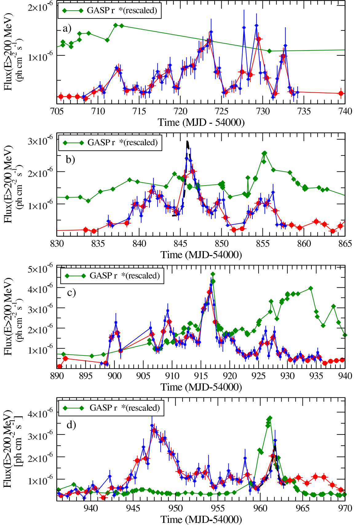
Fig. 2.— from top to bottom, flare a , b , c , and d showing 1-day binning (red points) and 12 hr binning (blue points). The green line is the rescaled data in the E > 200 MeV. The black shaded
