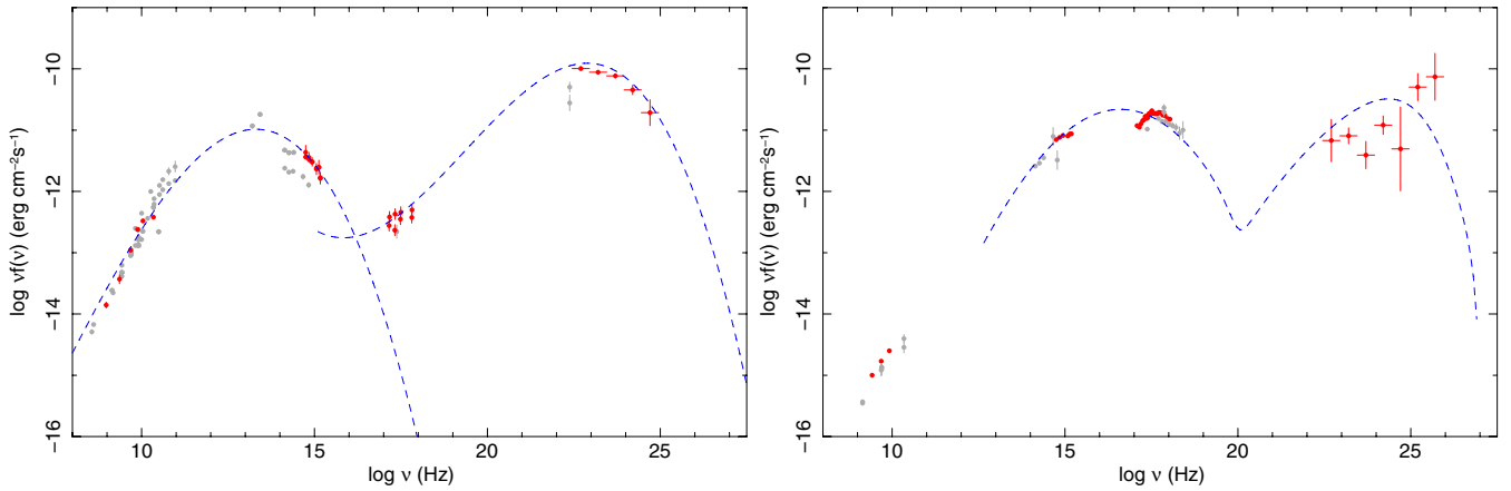
Figure 7. SED of 0FGL J0457.1–2325 = PKS0454-234 (left) and of 0FGL J0507.9+6739 = IES 0502+675 (right). (A color version of this figure is available in the online journal.)
