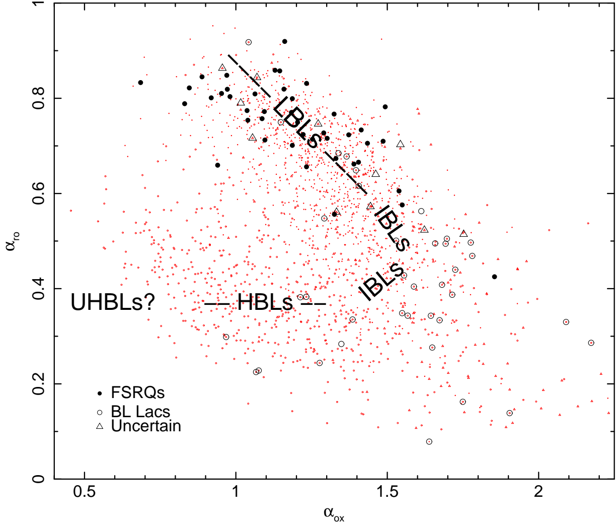
Fig. 27.— The \alpha_{\text{ox}} - \alpha_{\text{r0}} plot of the LBAS blazars (large symbols) compared to the sample of blazars in the BZCAT catalog for which there is radio optical and X-ray information (small red symbols). All gamma-ray selected blazars are located in regions covered by previously known blazars. No new \gamma -ray type of blazars has been found, in particular there is no evidence for thy hypothetical population of Ultra High energy peaked blazars (UHBLs), with synchrotron peak in the \gamma -ray band ( \text{Log}(\nu_{\text{peak}}^S) > 10^{20} Hz).
