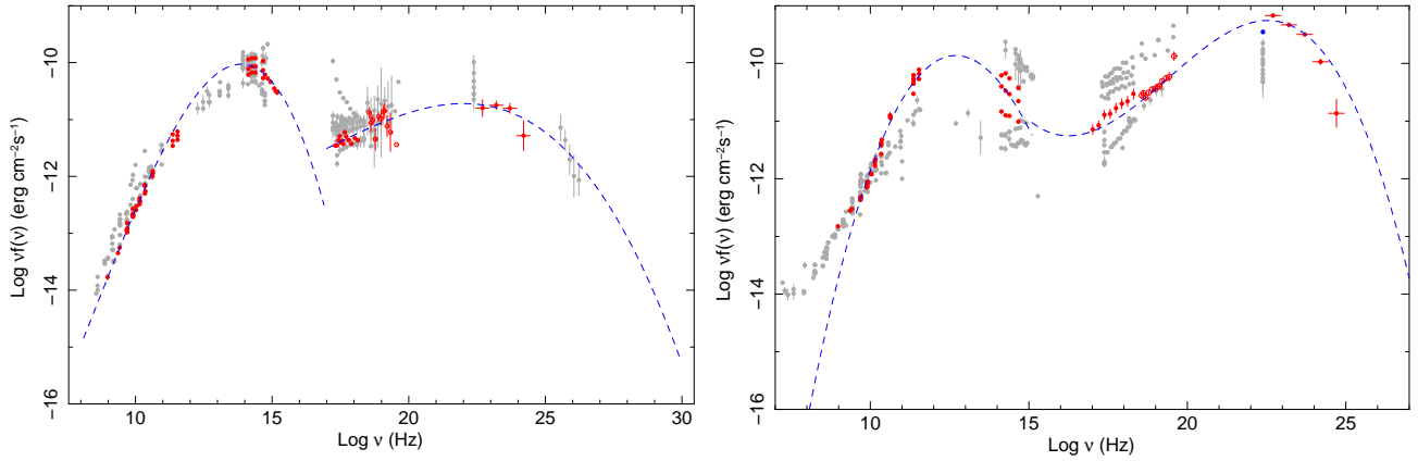
Fig. 23.— The SED of 0FGL J2202.4+4217 = BL Lacertae (left) and of 0FGL J2254.0+1609 = 3C454.3
