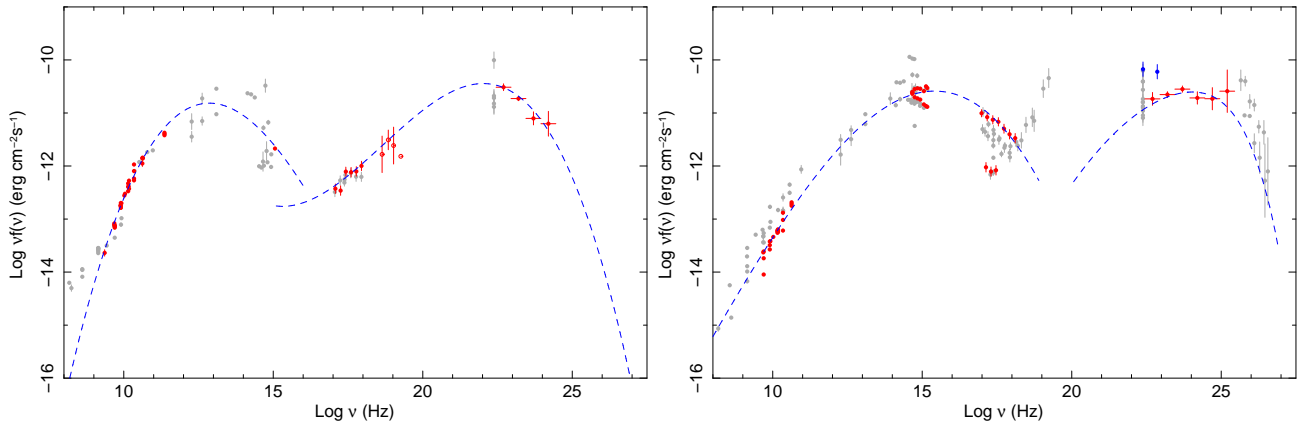
Fig. 14.— The SED of 0FGL J1159.2+2912 = 4C29.45 (left) and of 0FGL J1221.7+2814 = ON231 = W Comae (right)
