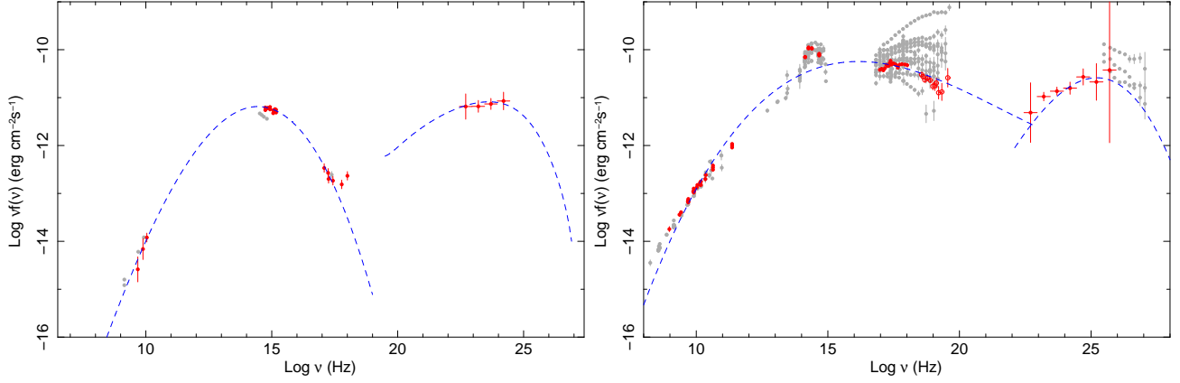
Fig. 19.— The SED of 0FGL J1543.1+6130 = GB6 J1542+6129 (left) and of 0FGL J1653.9+3946 = Mkn 501 (right)
