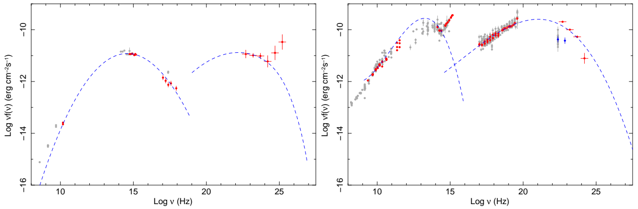
Fig. 15.— The SED of 0FGL J1248.7+5811 = PG 1246+586 (left) and of 0FGL J1229.1+0202 = 3C273 (right)
