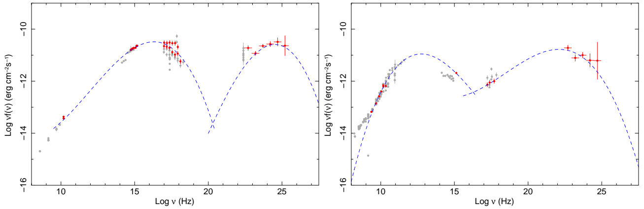
Fig. 12.— The SED of 0FGL J1015.2+4927 = 1H 1013+498 (left) and of 0FGL J1057.8+0138 = 4C01.28 (right)
