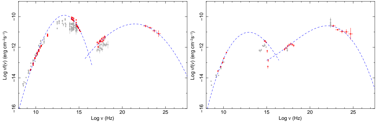
Fig. 11.— The SED of 0FGL J0855.4+2009 = PKS0851+202 (left) and of 0FGL J0921.2+4437 = S40917+44 (right)
