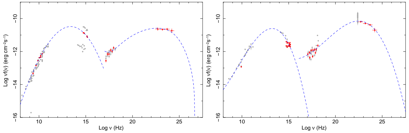
Fig. 2.— The SED of 0FGL J0137.1+4751 = S40133+47 (left) and of 0FGL J0210.8-5100 = PKS0208-512 (right)
