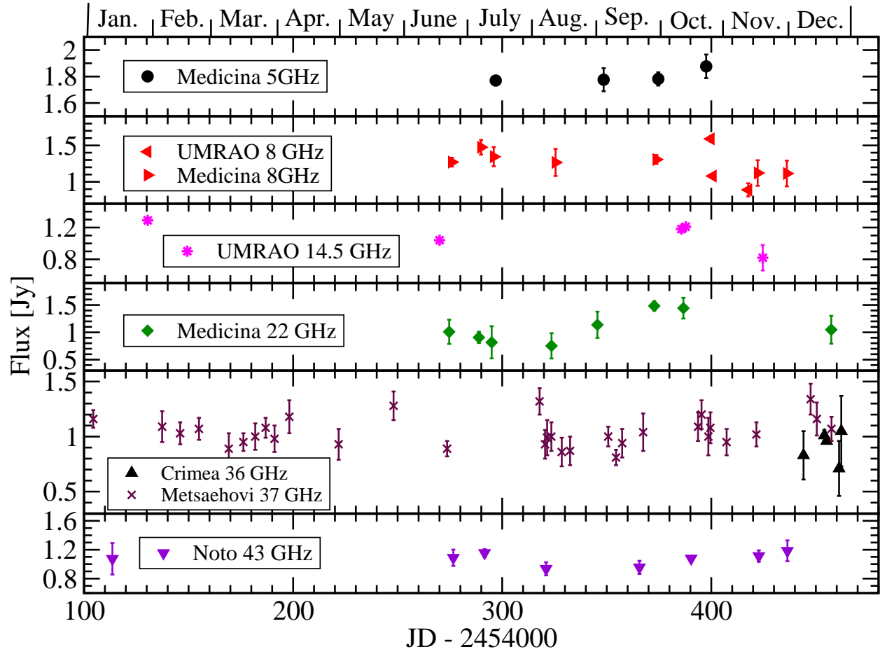
Fig. 6.— Radio light curves of 3C 66A in 2007.
