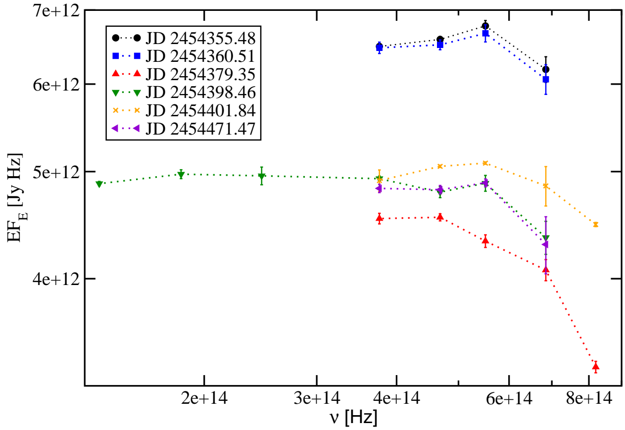
Fig. 7.— Intrinsic (after extinction correction) optical – near-IR spectral energy distributions during 6 epochs throughout the campaign.
