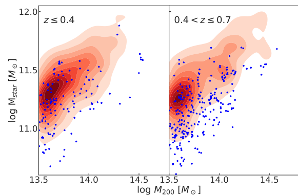
Figure 16. BCG stellar masses vs. cluster masses in the Illustris TNG300-1 sample: red contours display the distribution for red BCGs, values for blue BCGs are plotted as blue stars.
