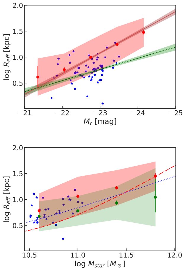
Figure 12. Top: size-luminosity distribution in BCGs. The wide area (light red) shows the 1-\sigma scatter for observed values, whose bootstrapped average values and error bars, and linear fits, are plotted in red. Values for blue BCGs are displayed as blue stars. The linear fits for galaxies with a low membership probability are displayed in green; shaded areas display 95% confidence intervals. Bottom: the size-stellar mass is displayed for BCGs with 0.3 < z < 0.5 (same symbols as above) and compared with the fits at z \sim 0.4 derived by Roy et al. (2018) for spheroid (dashed-dotted red) and disc (dotted blue) galaxies. The wide green area shows the 1-\sigma scatter for low membership probability galaxies.
