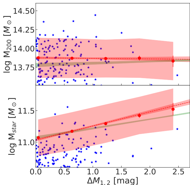
Figure 14. Total cluster mass (top panel) and stellar mass (bottom) as a function of the magnitude gap. The wider area (light red) shows the 1\text{-}\sigma scatter for observed values, whose bootstrapped average values and error bars are plotted as red circles. Blue BCGs are displayed as blue stars. The fits derived from the Illustris TNG300-1 simulations are marked in green. Shaded areas display 95% confidence intervals.
