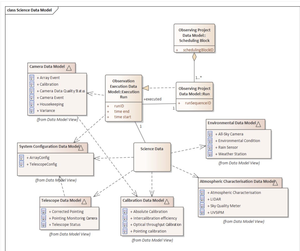
Figure 3: Science Data Model.
