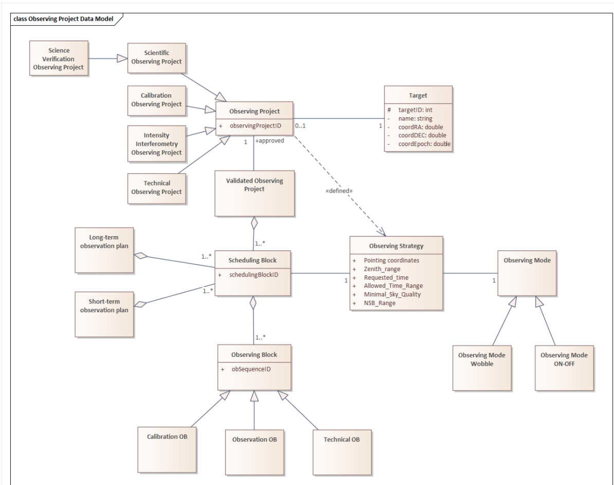
Figure 4: Observing Project Data Model hierarchy.
