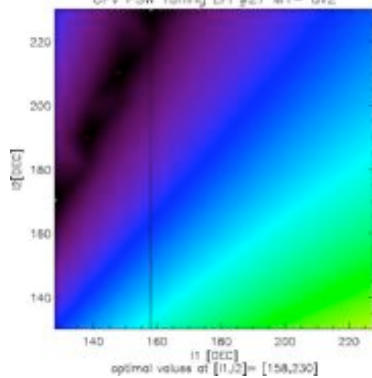
CPV PSW Tuning LFI #27 M2- \text{Sqrt}[(dV1)^2+(dV2)^2]
