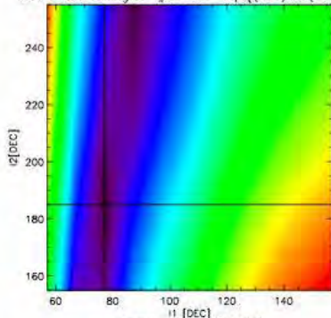
CPV PSW2 Tuning LFI #24 M2- \text{Sqrt}[(dv1)^2+(dv2)^2]
