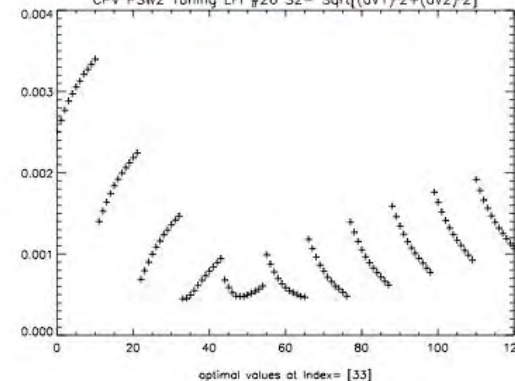
CPV PSW2 Tuning LFI #26 S2- \text{Sqrt}[(dV1)^2+(dV2)^2]
