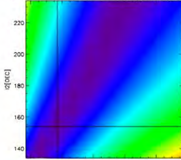
CPV PSW2 Tuning LFI #27 S1- \text{Sqrt}[(dv1)^2+(dv2)^2]
