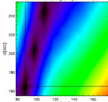
CPV PSW2 Tuning LFI #24 M1- dv1
