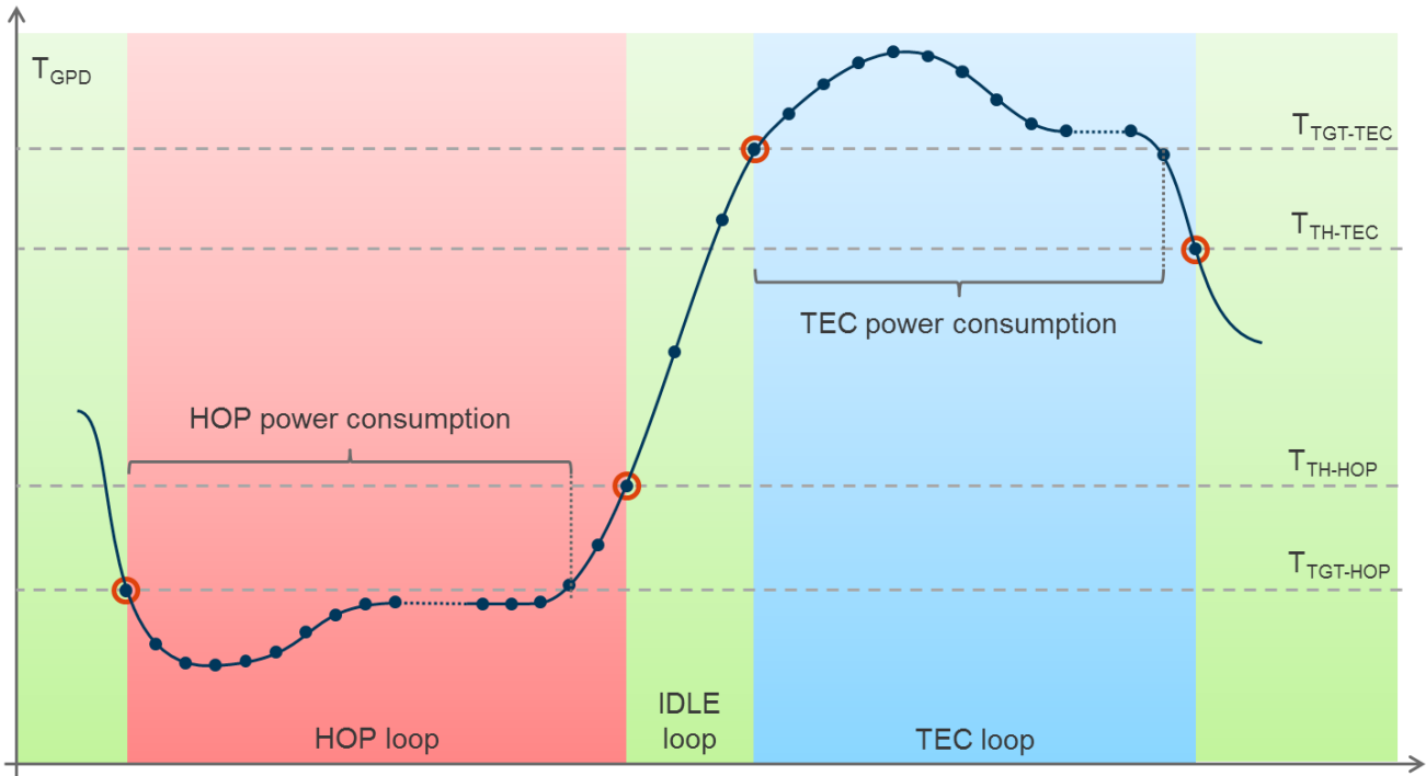
Figure 5-2: Thermal Control
