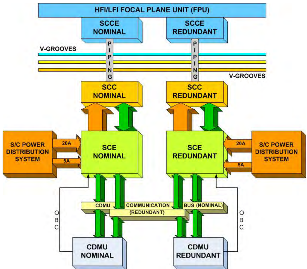
Figure 2-6 Block Diagram of the Sorption Cooler Electronics (SCE) configuration and redundancy with respect to the TMU and S/C (Full internal harness not shown)
