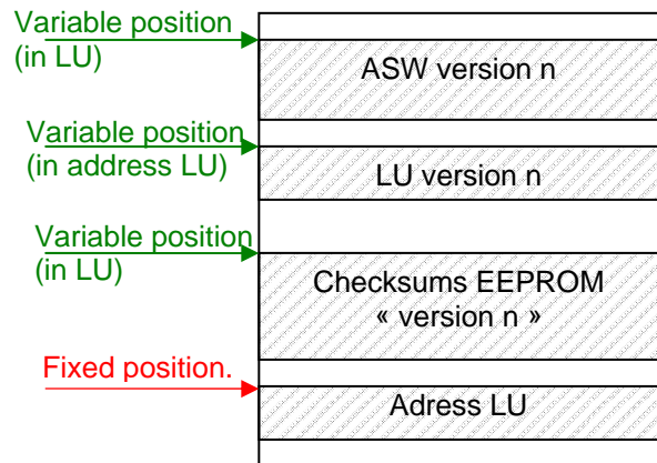
Figure 8-26: Eeprom configuration
