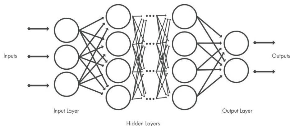
Fig. 5: Neural network
