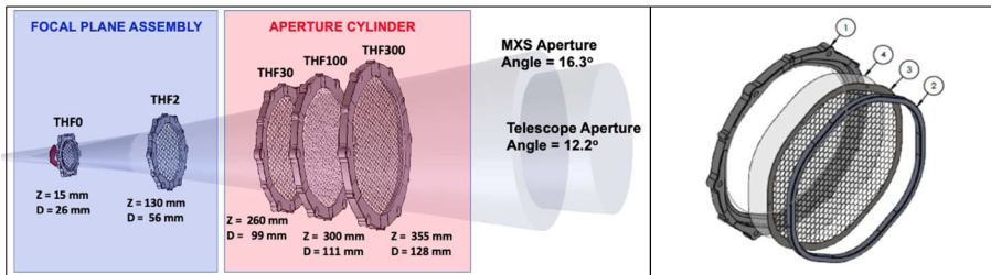
Fig. 15 Left) The stack of thermal filters located in the X-IFU field of view. Three filters have interfaces with the cryostat through the aperture cylinder, and 2 filters (the coldest) are located in the FPA. Right) THF300 schematic mounting of the film and supporting mesh inside the two-parts type frame. ① is the outer frame, ② is the inner frame, ③ is the supporting mesh and ④ is the thin polyimide/Al foil
