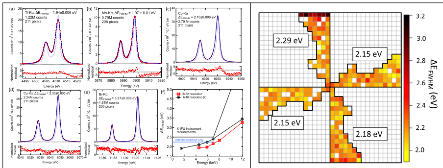
Fig. 21 Left From [31] Co-added 8-column by 32-row spectra for (a) Ti-K \alpha , (b) Mn-K \alpha , (c) Co-K \alpha , (d) Cu-K \alpha and (e) Br-K \alpha (measured from K-Br). The red dots are the data points, the light blue lines are the natural lines shapes and the dark blue line is the fit to data. The fitted \Delta E (Full Width at Half Maximum, FWHM), number of counts and number of pixels included in each spectrum are shown on the figures (f) \Delta E FWHM as a function of energy for the 1-column by 40-row measurements [41] and the new 8-column by 32-row results (red squares). The improved \Delta E FWHM is attributed to lower noise, improvements in the dynamic behavior of the readout chain and more optimized TES bias point. The dashed black line shows the X-IFU instrument level resolution requirements, and the dashed blue line shows the currently assumed requirements considering only the detector and readout subsystem and excluding margin. Right) From [31] \Delta E FWHM array heat map measured at Co-K \alpha
