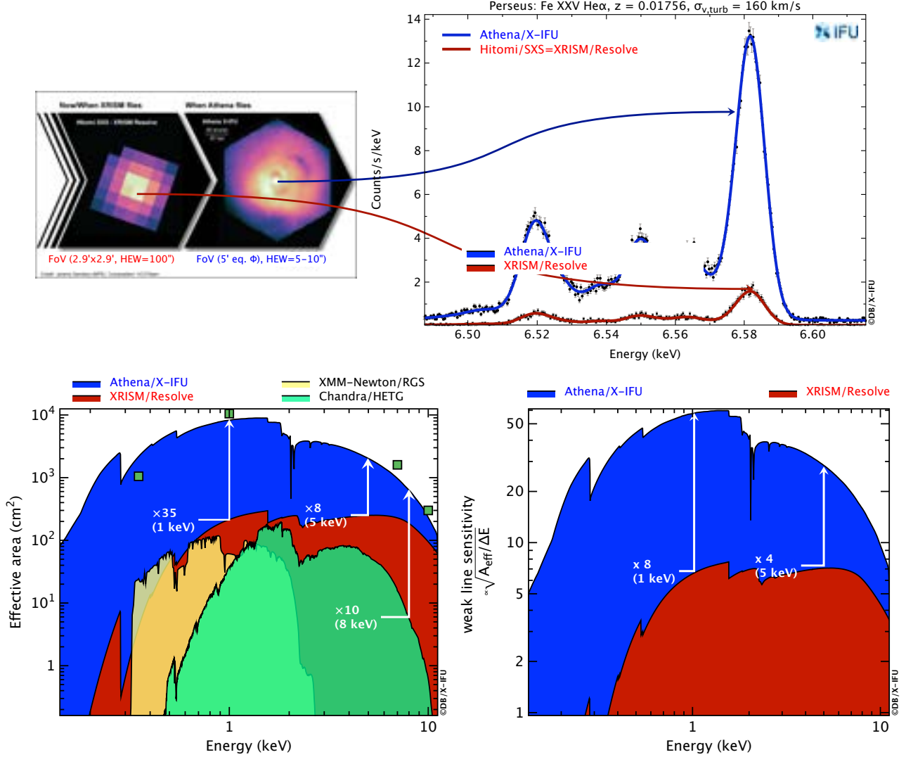
Figure 4. Top) The Hitomi/SXS=XRISM/Resolve and X-IFU images and spectra of Perseus cluster. Credit: Jeremy Sanders (MPE). This combined figure shows at the same time the significant improvement in fine imaging, over a comparable field of view, as well as the higher throughput of X-IFU compared to Resolve (the two spectra are simulated with the same exposure time). Bottom) Effective area (left) and weak narrow line sensitivity (right) of X-IFU in comparison with the one of XRISM/Resolve and Chandra/XMM-Newton gratings (not encapsulated in that figure, the fact that the angular resolution will be ten times better for Athena/X-IFU compared to XRISM/Resolve). The effective area requirement applying to X-IFU are indicated with filled green square symbols. This assumes the mirror telescope configuration as described in ATHENA - Telescope Reference Design and Effective Area Estimates, ESA-ATHENA-ESTEC-PL-DD-001, Issue 3.3, 21/12/2020 and the instrument efficiency presented in §4.1.
