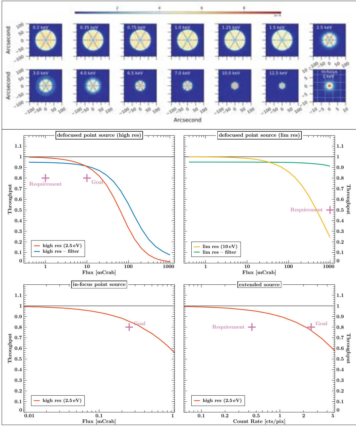
Figure 22. Top: The defocused PSF of the Athena optics at 13 energies as seen by X-IFU. 76 The bottom rightmost panel shows the in-focus PSF at 1 keV (Half Energy Width = 5"), for comparison. The grid in this panel shows the X-IFU pixels. We note that the in-focus PSF is shown on a 20" x 20" image while the defocused PSF is shown on a 200" x 200" image. The full field of view of the X-IFU is of the order of 300" (equivalent diameter). Bottom: Summary of the throughput performance for all the observing cases specified in the X-IFU URD. Requirements and goals are shown with crosses. Top left: High resolution observation of a defocused point source. Top right: Limited resolution (10 eV) observation of a defocused point source (for the filter configuration, the plot includes the 5 % loss due to the limited transmission of the beryllium filter in the 5 to 8 keV band of interest). Bottom left: High resolution observation of a focused point source. Bottom right: High resolution observation of an extended source.
