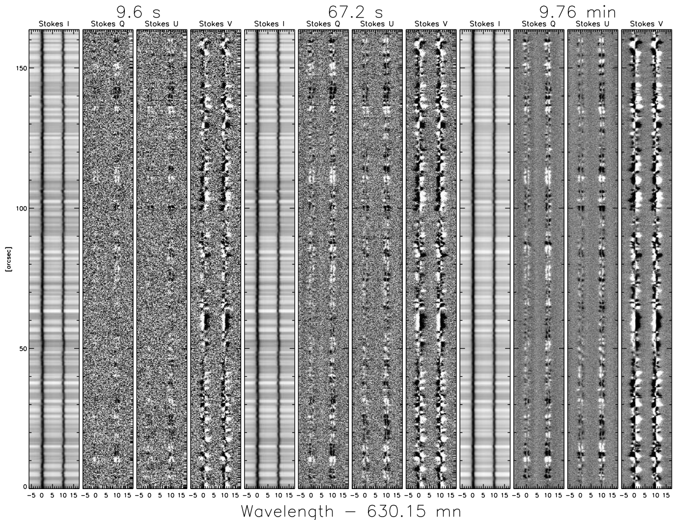
Fig. 2. Stokes I , Q , U , and V spectra of the two Fe I lines at 630 nm recorded by the Hinode spectropolarimeter in a quiet Sun region with integration times of 9.6 s ( left ), 67.2 s ( centre ), and 9.8 min ( right ). The Stokes Q , U , and V panels are saturated at \pm 10^{-3} I_{0s} . The linear polarisation signals (Stokes Q and U ) stand out more prominently over the slit the longer the integration time, (i.e. as the noise decreases). From Bellot Rubio & Orozco Suárez (2012) .
