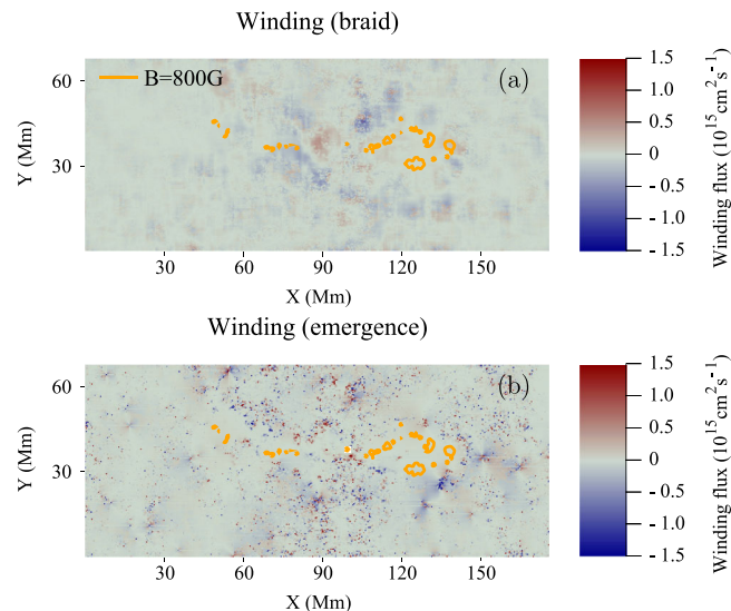
Fig. 4 Winding flux distributions of AR11318 during the plateau phase. Distributions of (a) dL_{\text{braid}}/dt and (b) dL_{\text{emergence}}/dt of AR11318 at t = 78 h. The orange contours indicate a field strength of B_z = 800 G. X and Y are distances along the x- and y-directions.
