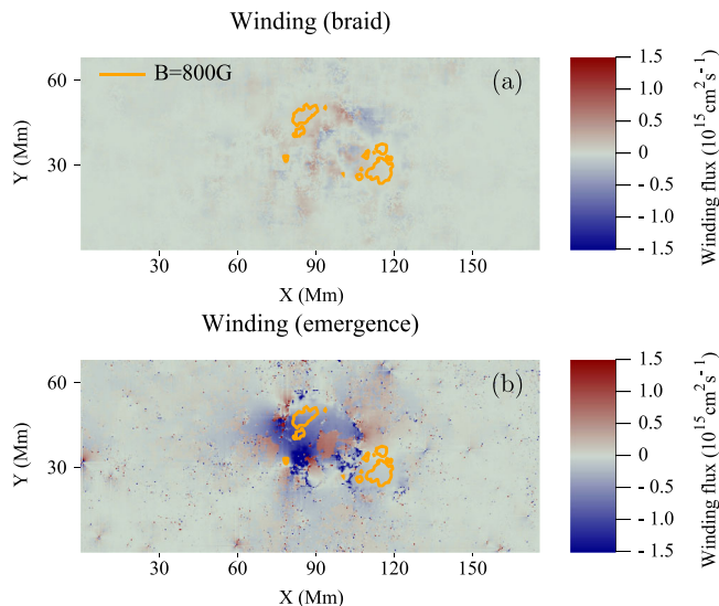
Fig. 3 Winding flux distributions for AR11318 during the rise phase. Distributions of (a) dL_{\text{braid}}/dt and (b) dL_{\text{emergence}}/dt of AR11318 at t = 42 h. The orange contours indicate a field strength of 800 G (and thus indicate the sunspot locations). X and Y are distances along the x- and y-directions.
