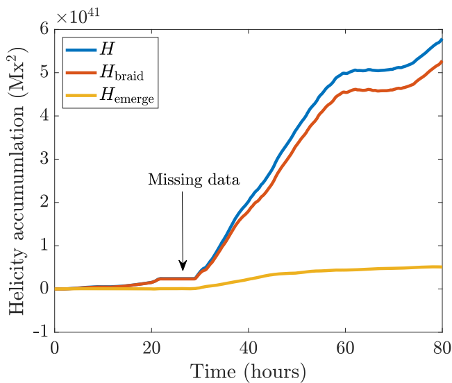
Fig. 6 Helicity accumulation for AR11318. The emergence accumulation H_{emerge} (yellow line), the braiding accumulation H_{braid} (red line), and the total helicity accumulation H = H_{emerge} + H_{braid} (blue line) are displayed. Source data are provided as a Source Data file.
