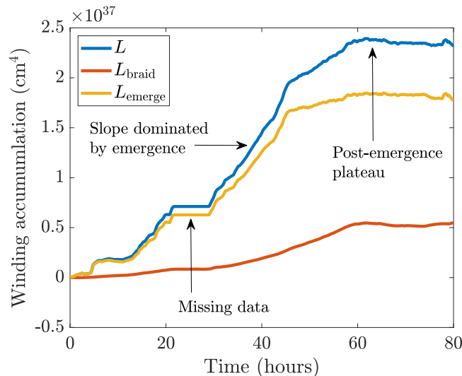
Fig. 2 Winding accumulation for AR11318. The emergence accumulation L_{\text{emerge}} (yellow line), the braiding accumulation L_{\text{braid}} (red line), and the total winding accumulation L = L_{\text{emerge}} + L_{\text{braid}} (blue line) are displayed. The missing data are between t = 20 and t = 30 h. Source data are provided as a Source Data file.
