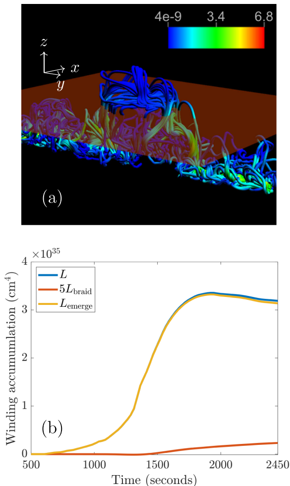
Fig. 1 Simulation of the initial emergence of a twisted magnetic tube. (a) displays field lines at t = 2500 s, with a slice indicating the horizontal photospheric boundary (red plane) where the magnetic field is measured. The x , y - and z -directions are indicated. The colour bar indicates (dimensionless) magnetic field strength (to convert to physical units, see Methods: Numerical simulation details). Darker colours (mainly blue) indicate weaker field strengths and lighter colours (green and yellow) indicate stronger field strengths. In (b), the emergence accumulation L_{\text{emerge}} (yellow line), the braiding accumulation L_{\text{braid}} (red line), and the total winding accumulation L = L_{\text{emerge}} + L_{\text{braid}} (blue line) are displayed. 5 \times L_{\text{braid}} is displayed on the figure in order to convey clearly how L_{\text{braid}} develops in time.
