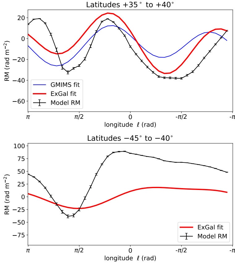
Figure 20. Constant latitude binned slices through the -M0-M1 model. The upper panel covers latitudes +35^\circ < b < +40^\circ , the red and blue curves are copied from the upper panel of Fig. 2. The lower panel is for -45^\circ < b < -40^\circ corresponding to Fig. 6. Error bars show the scatter of values in each longitude bin, which are necessarily small because of the low angular resolution of the model.
