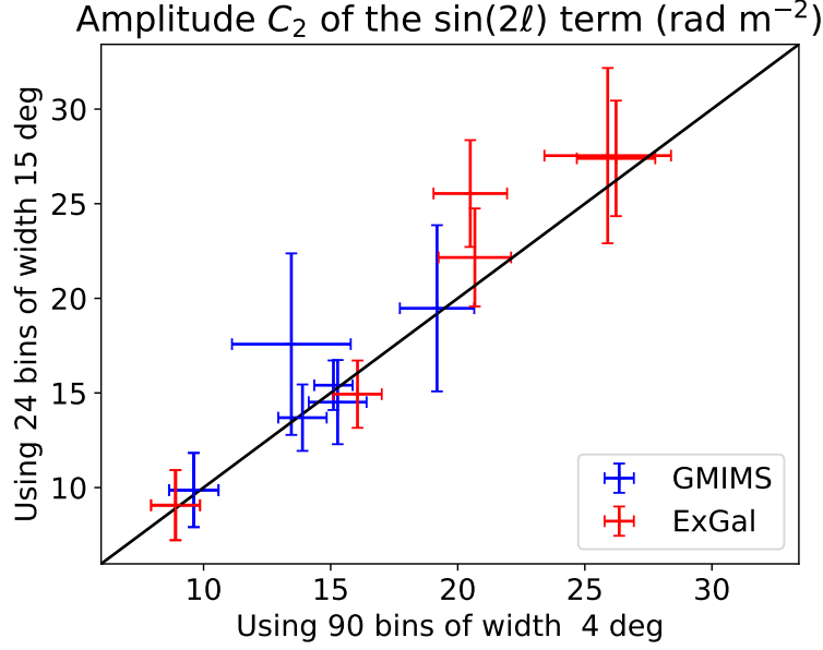
Figure 23. Comparing the fitted values of coefficient C_2 (Eq. 1) at different latitudes for different bin widths, 4^\circ and 15^\circ , as on Fig. 22. Only latitudes giving values of C_2 > 5\sigma are shown. For all but one point the results agree within error bars of \pm 1\sigma . From this and similar comparisons with many different bin widths, we conclude that the bin size has minimal effect on the least squares fitting in section 2.
