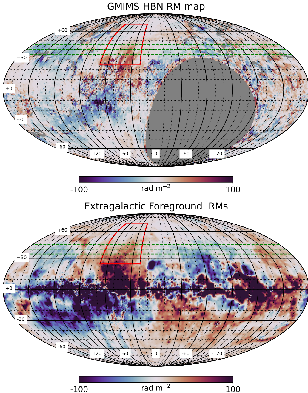
Figure 1. Two maps of the Galactic RM. The upper panel shows the GMIMS High Band North first moment map made with data from the DRAO 26m telescope (Wolleben et al. 2021). The lower panel shows the Galactic estimate based on extragalactic source RMs (Hutschenreuter et al. 2022). The red box indicates the area dominated by the North Polar Spur in Stokes I synchrotron emission, see Section 2.3 below. The green dashed lines illustrate two sets of bins at constant latitude, used to make the two panels on Fig. 2.
