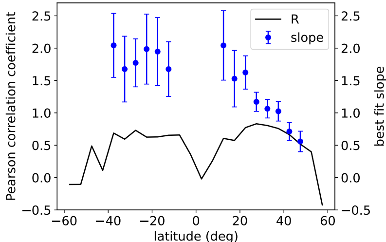
Figure 5. The Pearson correlation coefficient, R , versus Galactic latitude, from Table 2. The blue dots show the slope, \frac{\Delta RM_{ExGal}}{\Delta RM_{GMIMS}} , of the best fit line (right hand axis). Dots are plotted only for latitudes 10^\circ < |b| < 50^\circ where the correlation is strong ( R > 0.5 ).
