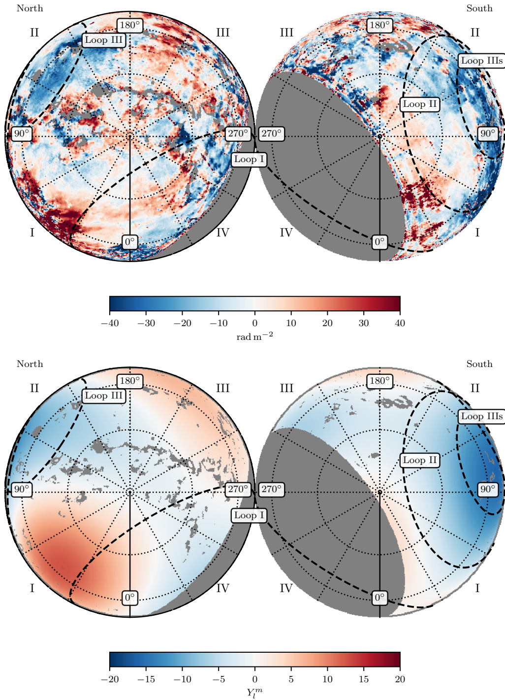
Figure 16. The upper panels show the Wolleben et al. (2021) map of the GMIMS RMs in orthographic projection. The lower panels show the spherical harmonic expansion, as on Fig. 15. The radio continuum loops discussed in the text are indicated as on Fig. 15. The grey patches are areas where the signal-to-noise is too low to allow calculation of the first moment of the Faraday spectrum.
