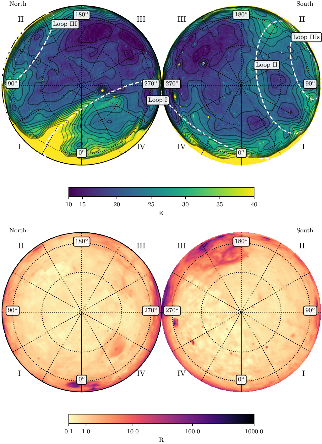
Figure 17. The upper panels show Stokes I emission at 408 MHz (de-stripped) (Haslam et al. 1982; Remazeilles et al. 2015). The lower panels show the H \alpha emission from SHASSA, VTSS, and WHAM (Finkbeiner 2003). Alignment and overlays are the same as Fig. 15.
