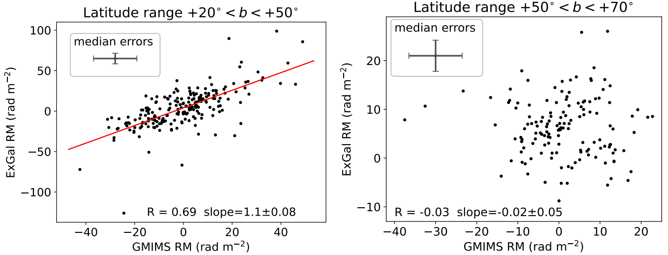
Figure 4. Scatter plots of median values from the extragalactic RM map of Hutschenreuter et al. (2022) versus corresponding median values of RM from the GMIMS survey for the latitude range +20^\circ < b < +50^\circ (left panel) and +50^\circ < b < +70^\circ (right panel). On the left, the correlation coefficient is R=0.69 , and the slope of the best fit line is 1.1 \pm 0.08 , whereas on the right there is no correlation ( R = -0.03 ). The median errors on the points are shown in the insets. On the right (high latitudes) the standard deviation of the GMIMS values is 9.8 (x axis) and for the extragalactic values the standard deviation is 6.1 (y axis).
