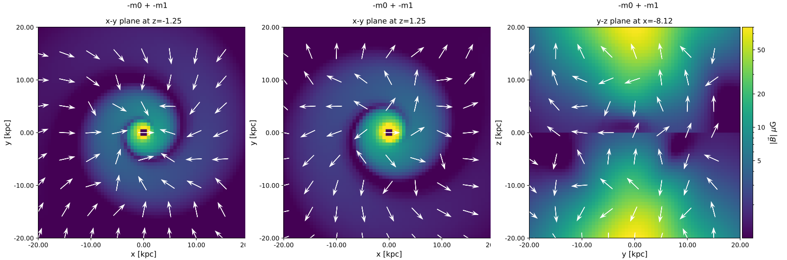
Figure 21. Examples of the \vec{B} field configuration in the -M0 (dipolar) -M1 (quadrupolar) model. The left and middle panels show the field direction projected on planes parallel to the midplane, displaced above and below midplane by 1.25 kpc. The right panel shows the field on a plane perpendicular to the midplane, through a position ( x = -8.1 kpc, y = 0 , z = 0 ) normal to the radial direction, roughly corresponding to the position of the observer for the computation of the RM figures 18, 19, and 20. The \vec{B} field model is for a generic spiral galaxy, it has not been fitted to the Milky Way, so the scales on the axes are representative. Unlike Figs. 18, 19 and 20, the field is not integrated along the line of sight nor projected on the sky, these panels merely illustrate sections through the model. The background color shows the magnitude of the field ( |\vec{B}| ), with a logarithmic scale. The field is neither symmetric nor antisymmetric about the midplane.
