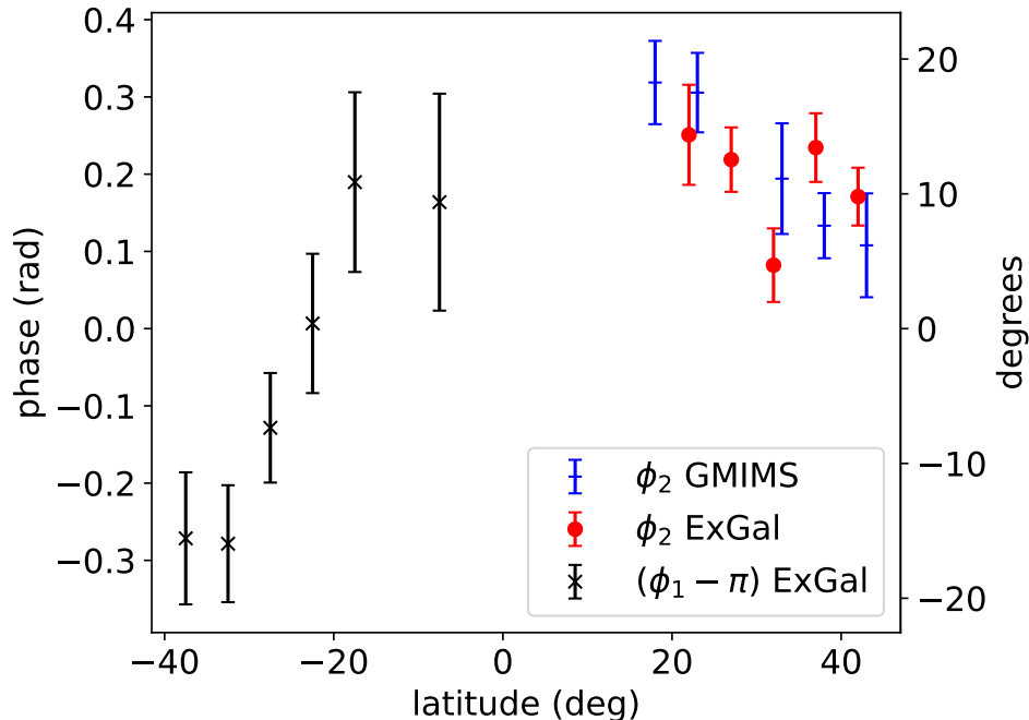
Figure 9. The fitted phases of the \sin \ell and \sin(2\ell) functions, i.e. \phi_1 and \phi_2 in Equation 1. In the Northern Hemisphere, \phi_2 from both the GMIMS and the extragalactic fits are shown, in blue and red respectively. In the South, the extragalactic fits give \phi_1 \simeq \pi . In the figure we subtract \pi to get the black points on the same scale as the \phi_2 values in the North. Note that both the error bars and the range of values for \phi_1 naturally have about twice the range as for \phi_2 because of the factor of two in the third term on the right of Eq. 1. The conditions for including points on the plot are that R > 0.5 and the error in \phi is small, i.e. \sigma_{\phi_2} < 0.075 radians or \sigma_{\phi_1} < 0.15 radians.
