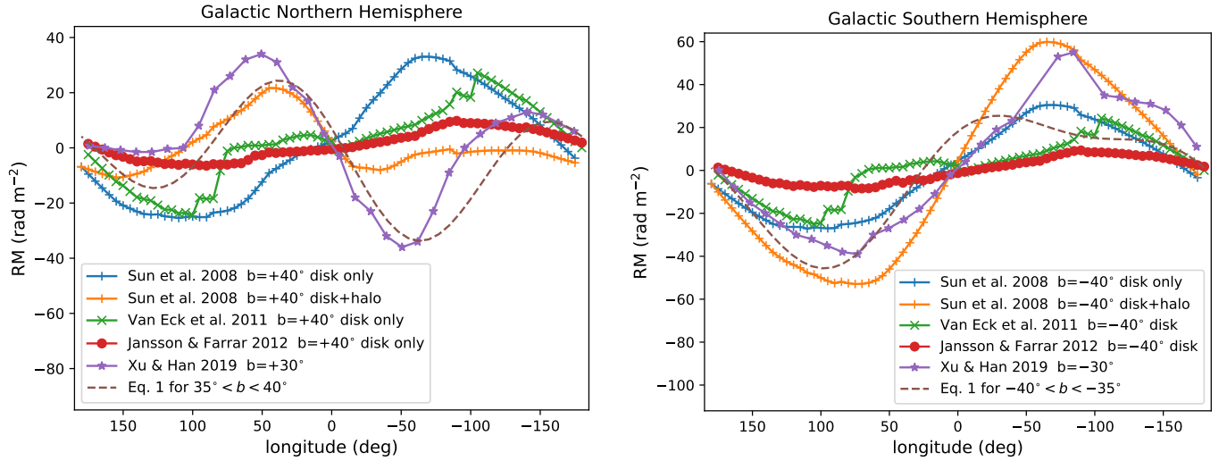
Figure 14. Models for the contribution of the disk to the RMs observed at intermediate latitudes. The left panel shows North latitudes ( b = +40^\circ ) and the right panel shows the corresponding south latitudes ( b = -40^\circ ). These are computed following the method described in Ma et al. (2020, sec. 2.2) . The blue and orange curves result from the model of Sun et al. (2008) for the disk component and disk plus halo, respectively. The green curve is the disk component of the Van Eck et al. (2011) model, and the red is the disk component of the model by Jansson & Farrar (2012) . The recent model of the halo contribution to RMs of pulsars Xu & Han (2019) is shown in purple for b = \pm 30^\circ (copied from their Fig. 17). For comparison the Equation 1 fits to the extragalactic RMs for similar latitude ranges are shown by the dashed curves. The Xu & Han (2019) halo model matches the models for the GMIMS and extragalactic RMs quite well in both hemispheres, as does the Sun et al. (2008) disk plus halo model, but the disk only models do not fit the RM pattern in the Northern Hemisphere.
