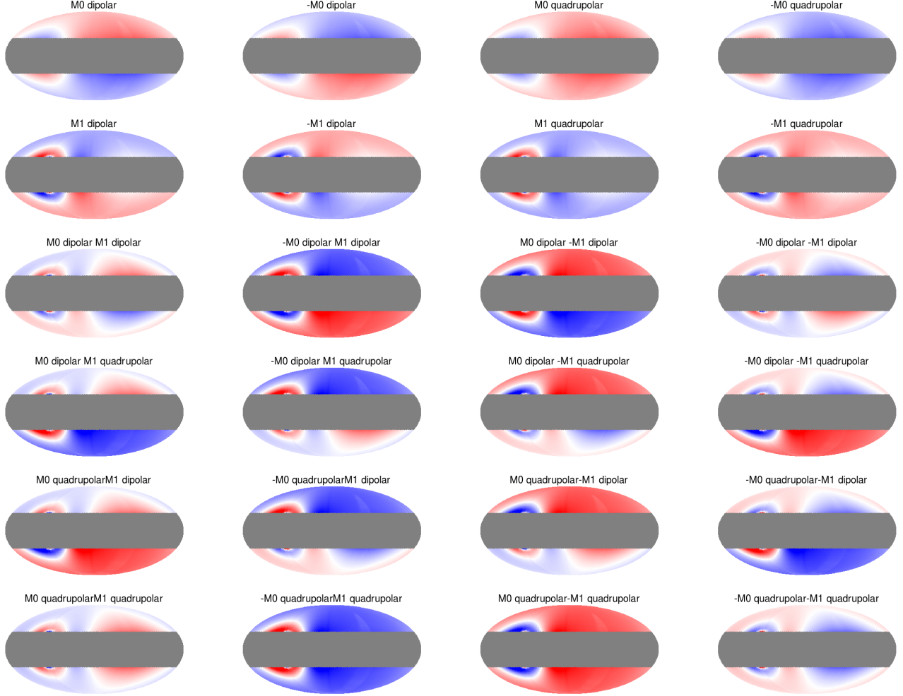
Figure 18. Simulated RM maps showing the M=0 and M=1 modes, each with \pm dipolar and quadrupolar symmetry. The two top rows show these modes individually. The lower rows show all 16 combinations thereof. The case of -M=0 dipolar added to -M=1 quadrupolar, in the fourth row and rightmost column, is reproduced in Fig. 19.
