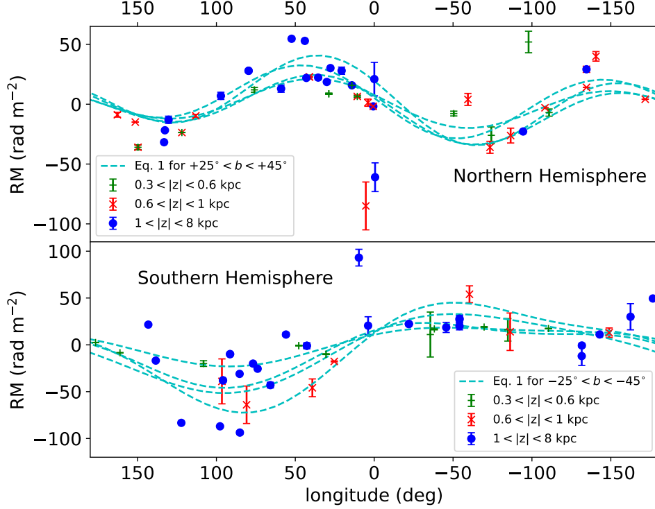
Figure 13. Rotation measure versus longitude for pulsars with latitudes +25^\circ \leq b \leq +45^\circ and z > 0.3 kpc (upper panel) or -25^\circ \geq b \geq -45^\circ and z < -0.3 kpc (lower panel). For comparison, the Eq. 1 predictions using the extragalactic fit parameters (Table 1) are indicated by the dashed curves. Many of the pulsars have such precisely measured RMs that the error bars are smaller than the symbols. In both hemispheres, the agreement between the extragalactic RMs and the pulsar RMs is very good, particularly for pulsars with |z| > 0.6 kpc.
