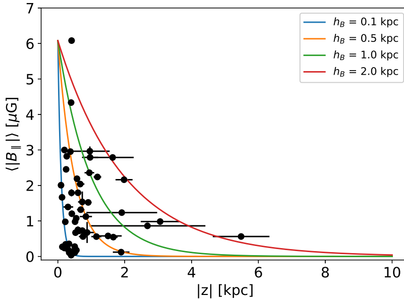
Figure 12. Correlation between the average LoS magnetic field, \langle B_{\parallel} \rangle , and |z| for our selected 54 pulsars. Four analytical trends of the form \langle B_{\parallel} \rangle = \langle B_{\parallel, 0} \rangle e^{-|z|/h_B} are overlaid as functions of the magnetic field scale height, h_B . As on Fig. 11, the points are scattered over a wide range, but they are mostly consistent with h_B < \sim 0.5 kpc.
