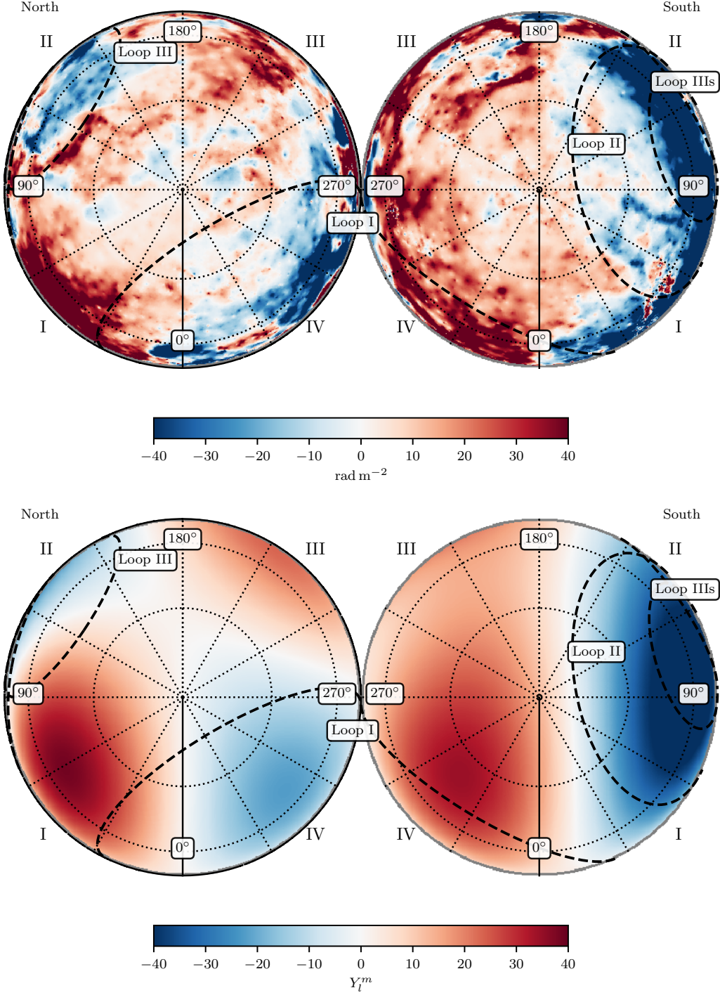
Figure 15. Upper: The extragalactic RM map of Hutschenreuter et al. (2022) in orthographic projection, centred on the Galactic poles. The left panel shows the Northern Hemisphere, the right panel shows the south, with circles of constant latitude at b = \pm 30^\circ and \pm 60^\circ . Lower: The spherical harmonic expansion of the Hutschenreuter et al. (2022) RM distribution with l_{\max} = 3 . We overlay the positions of nearby radio continuum loops ( Vidal et al. 2015 ) and label the Galactic quadrants by Roman numerals on both panels. As these are images of the sky, parity is reversed compared with the ordinary face-on view of the Galactic plane seen from above the Northern Hemisphere.
