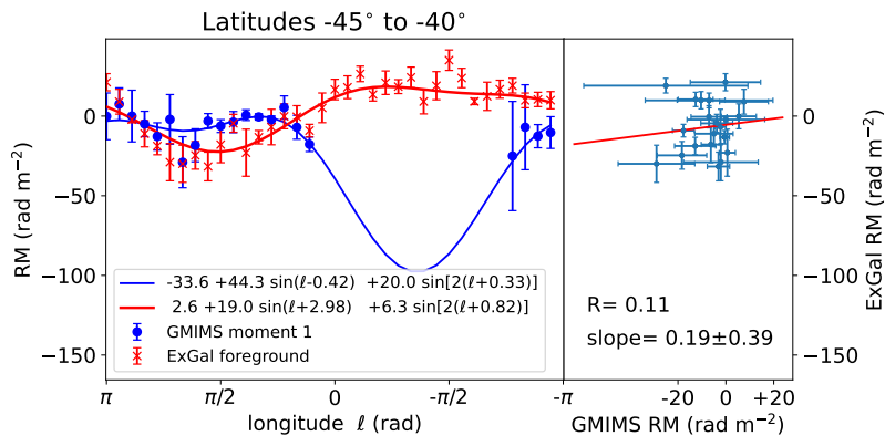
Figure 6. Comparison of GMIMS and extragalactic RMs at latitudes -45^\circ < b < -40^\circ . In this case the two surveys give roughly similar results in the first and second Galactic quadrants ( 0 < \ell < \pi ), but the GMIMS survey misses most of the third and fourth quadrants. The fitting is poorly constrained as a result, and the constants are ill determined. In addition, there is very little correlation between the RMs from the two surveys (right panel).
