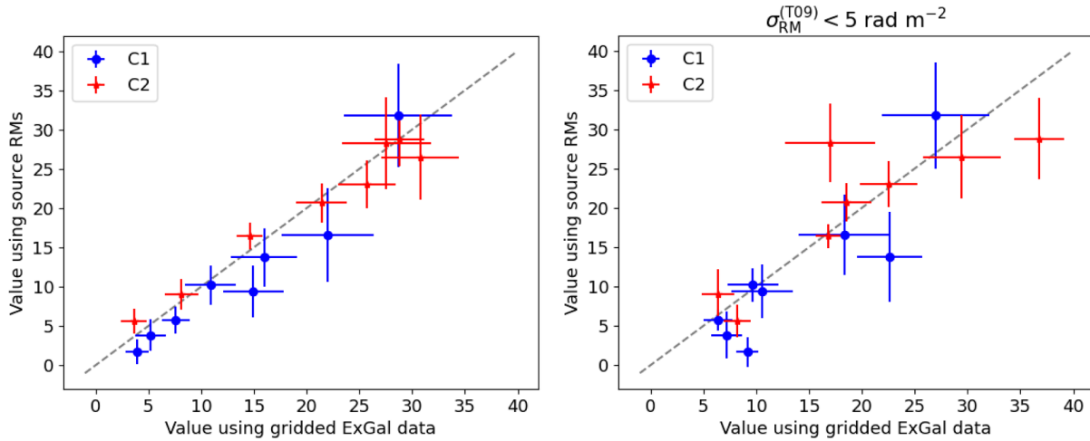
Figure 25. Comparing the fitted values of coefficient C_1 and C_2 (Eq. 1) at northern latitudes ( 15^\circ < b < 55^\circ ) for 10 degree bins using the gridded extragalactic RMs vs. binning the extragalactic sources directly from Taylor et al. (2009). The left panel uses all sources with equal weighting. The right panel uses only the sources with the highest precision in RM, i.e. those with measurement error \sigma_{RM} < 5 \text{ rad m}^{-2} .
