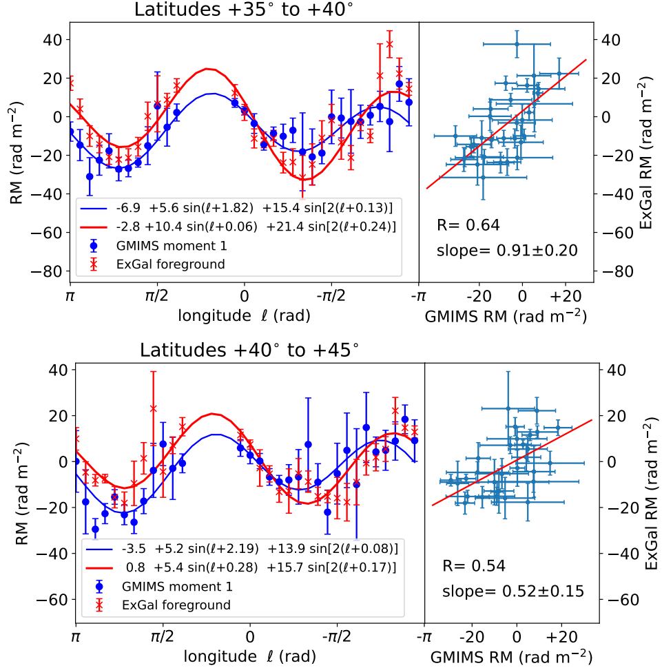
Figure 7. The effect of blanking an area that covers the bright emission region corresponding to the North Polar Spur ( 25^\circ < b < 70^\circ and 20^\circ < \ell < 70^\circ ). The latitude ranges are the same as those shown on Fig. 2
