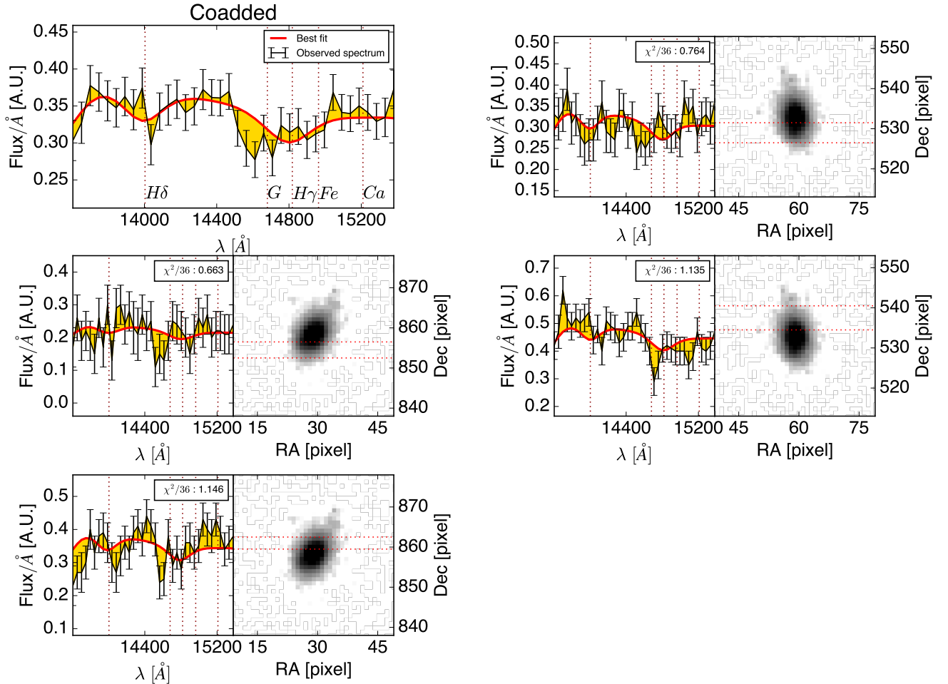
Fig. A.6: Same as Fig. A.1 for the outer zone of ID64.
