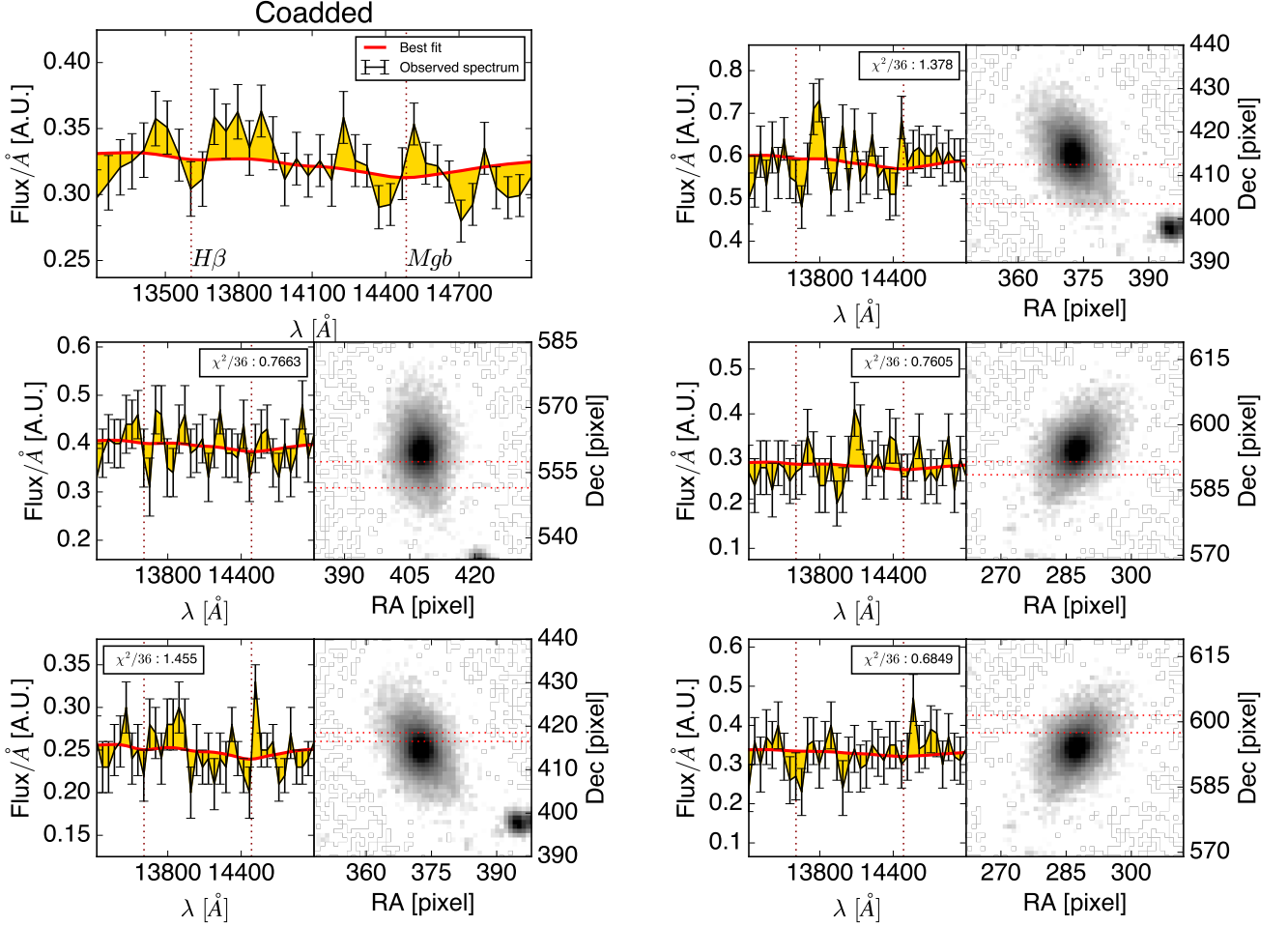
Fig. A.2: Same as Fig. A.1 for the outer zone of ID272.
