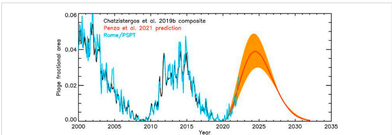
FIGURE 11 Prediction of solar cycle 25 amplitude in plage fractional areas by Penza et al. (2021, red, with confidence intervals in shaded orange surface). Shown also is the Chatzistergos et al. (2019b) plage area composite (black), on which the prediction was based, as well as more recent data from Rome/PSPT (light blue), which was the reference observatory in the Chatzistergos et al. (2019b) plage area composite since 1996.
