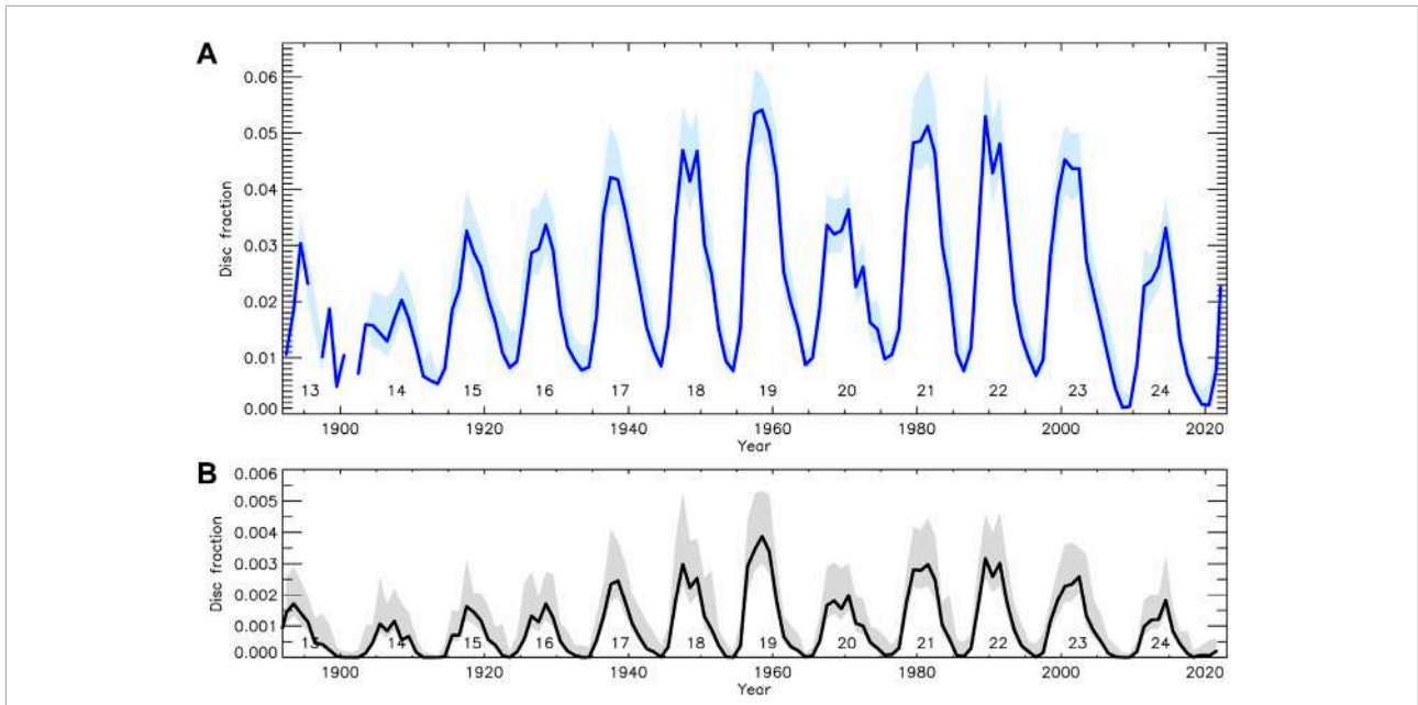
FIGURE 10 (A) Plage area composite series by Chatzistergos et al. (2020c) extended to 10 March 2022 with Rome/PSPT data processed in the same way as the rest of the data used for the composite series. (B) Sunspot area series by Mandal et al. (2020). Shaded areas mark the asymmetric 1\sigma intervals, while the numbers at the lower part of each panel denote the conventional solar cycle numbering.
