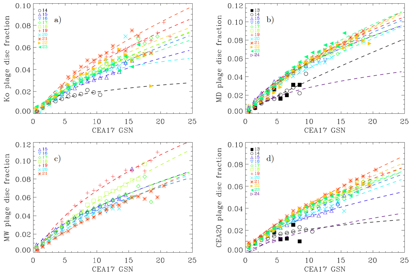
Fig. A.2. Relation between plate areas and CEA17 GSN for individual SC based on the data from the Ko (a), MD (b), and MW (c) archives as well as the CEA20 plate area composite (d). Shown are the binned values along with power law fits. The lines are coloured according to the strength of the SC with the strength increasing from black for the weakest cycle, via dark blue, turquoise, green, lime, orange, bright red to dark red for the strongest SC.
