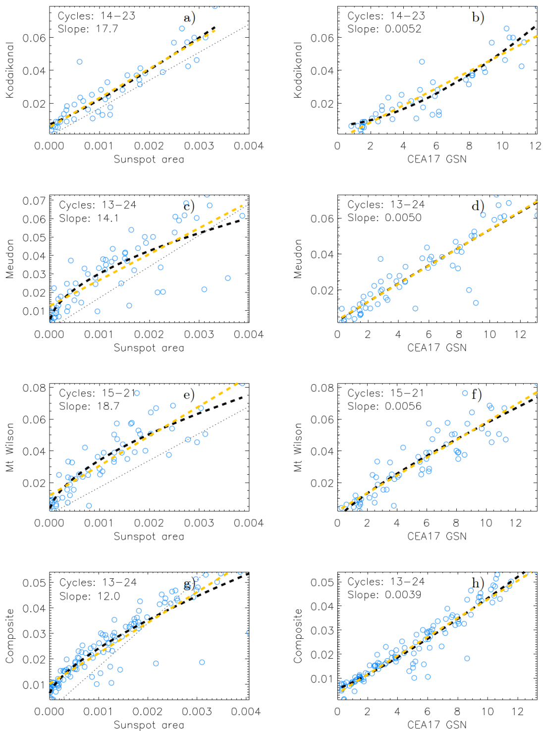
Fig. 2. Scatter plots between annual plage fractional areas and the annual MEA20 sunspot fractional areas (left columns) as well as the annual CEA17 GSN series (right columns). Two different fits are over-plotted, a power law (black) and a linear (yellow) fit. The dotted line has a slope of 17, which corresponds to the mean ratio between the CEA20 plage area series and the MEA19 sunspot area series (see Sect. 3.1). The period of overlap between the two archives (expressed in solar cycles) as well as the slope of the linear fit are shown in each panel.
