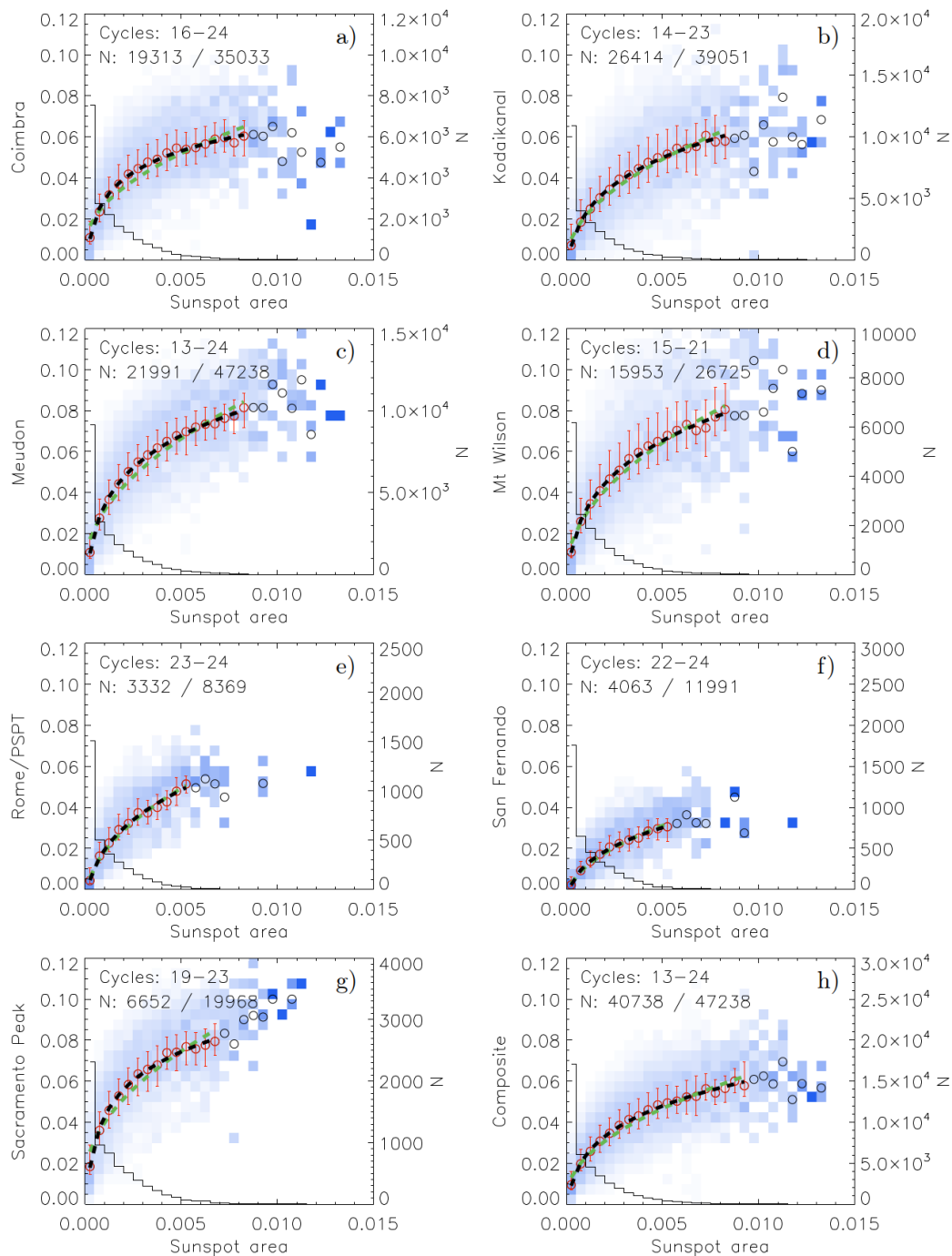
Fig. 1. Probability distribution functions (PDF) for plage fractional areas as a function of the sunspot fractional areas from MEA20. Both plage and spot areas were taken on the same days. The PDFs are shown in bins of 0.005 and 0.0005 fractional areas for plage and sunspots, respectively. Each panel shows the PDF matrix for a given Ca II K archive; Co (a)), Ko (b)), MD (c)), MW (d)), RP (e)), SF2 (f)), SP (g)), and the CEA20 plage area composite (h)). The PDFs are colour-coded between white for 0 and bright blue for 1. Circles denote the average plage area value within each column. For columns with less than 20 days of data these circles are shown in black, otherwise in red. We also show the asymmetric 1\sigma interval for each column. Two different fits to the average values are over-plotted, a power law fit (black), and a square root function (green). The number of days included in each column is also shown as a solid black histogram (see right-hand axis). The period of overlap between the two archives shown in a given panel (expressed in solar cycles), as well as the total number of overlapping days used to construct each matrix (N) and the total number of days within this time interval are listed in the top part of each panel.
