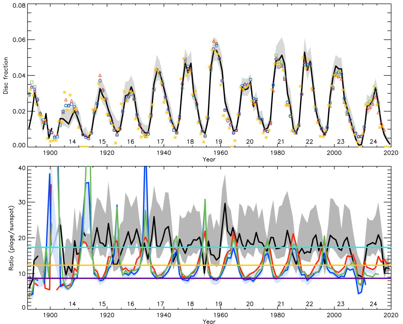
Fig. 4. Upper panel: CEA20 plage area composite (black line) along with scaled sunspot series by MEA20 (yellow asterisks), CEA17 (blue circles), ISNv2 (red triangles), and SvSc16 (green squares). All series are scaled linearly to the plage areas except MEA20 which is scaled with a square root function. The solid lines are annual median values while the grey shaded surface is the asymmetric 1\sigma interval. Lower panel: Ratio of the CEA20 plage areas composite to the sunspot area series by MEA20 (black) and sunspot number series by CEA17 (blue), SvSc16 (green), and ISNv2 (red) as a function of time. The ratios to the GSN series have been multiplied by 2000 to allow a direct comparison to the ratios to the sunspot areas. The blue shaded surface marks the range of annual values for the plage areas to sunspot number ratios from all sunspot number series used in this study. The ratios are calculated only for the days on which sunspot areas are greater than 0.0005 of the disc area or the sunspot number is greater than 0. The yellow (light blue) horizontal line marks the mean ratio of plage areas to sunspot numbers (sunspot areas), while the purple horizontal line is the mean ratio for the plage areas to sunspot number series over four-year intervals around cycle maxima. The numbers below the curves in each panel denote the conventional SC numbering and are placed at times of SC maxima.
