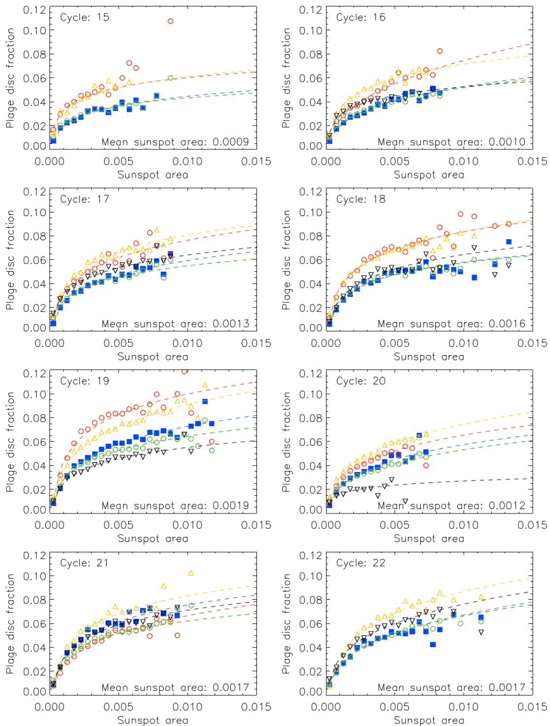
Fig. A.3. Similar to Fig. A.1, but now each panel shows the relationships for Co (black downward triangles), Ko (blue squares), MD (orange upward triangles), MW (red circles), and CEA20 composite (green circles) series for individual SCs 15 to 22, as specified in each panel. Also listed in each panel is the cycle-averaged sunspot fractional area.
