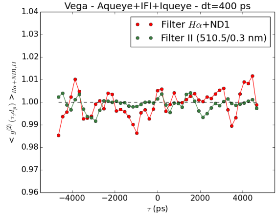
Figure 4. Temporal correlation on a \sim km baseline \langle g^{(2)}(\tau, d_p) \rangle_{\text{H}\alpha+\text{ND1,II}} for all the Aqueye+IFI+Iqueye Nov 2019 observations of Vega reported in Table 3 and for the two adopted combinations of filters, H \alpha +ND1 and II. The time bin is dt = 400 ps. Data is corrected for the light travel time delay between telescopes. The projected baseline d_p varied in the range 1535-2418 m.
